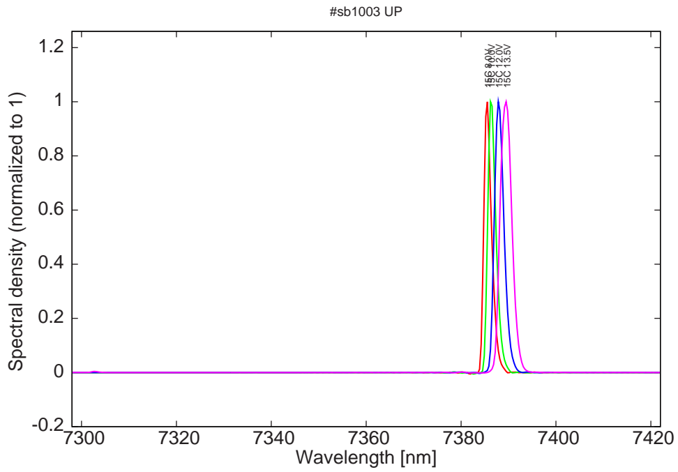
Figure 15: spectra at 15C for various LDD voltages (small mode around 7303nm at 13.5V on LDD)
