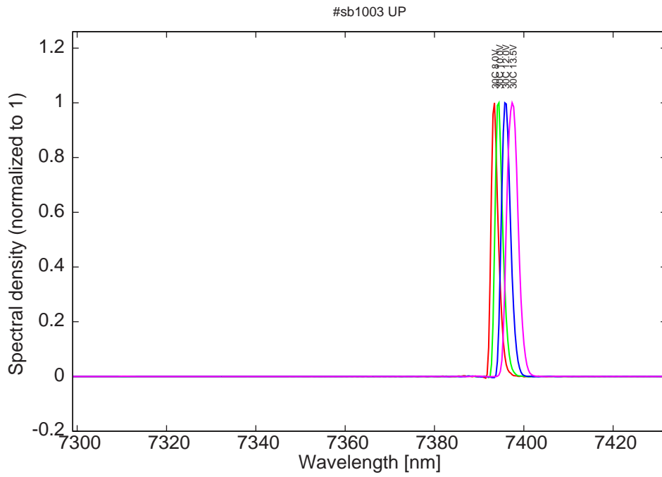
Figure 17: spectra at 30C for various LDD voltages (small mode around 7310nm at 13.5V on LDD)
