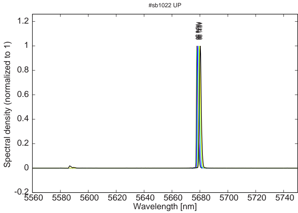
Figure 13: spectra at 0C for various LDD voltages
