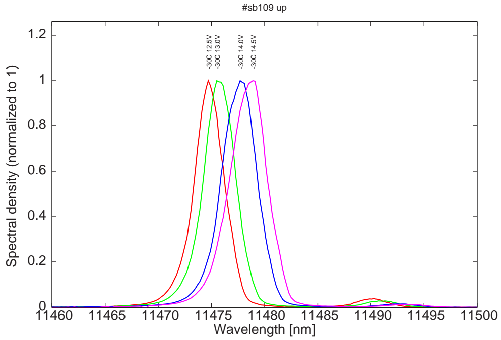
Figure 9: spectra at -30C at 2% dc for various LDD voltages (bimode)
