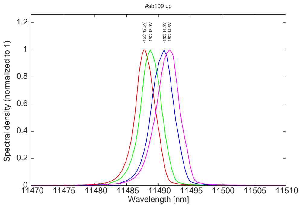
Figure 10: spectra at -15C at 2% dc for various LDD voltages
