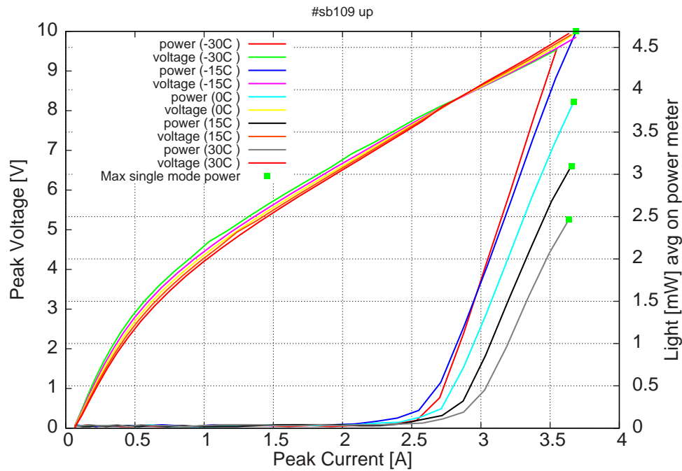
Figure 4: peak voltage and avg power vs peak current at 2% dc (the solid squares indicate the maximum singlemode emitted power)
