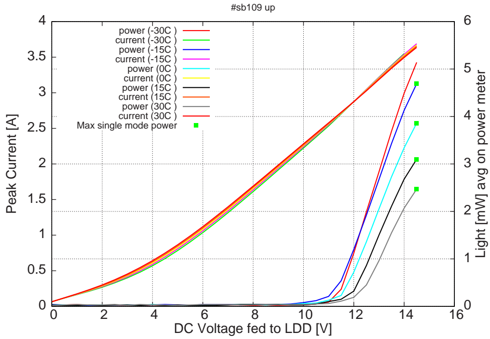
Figure 7: peak current and avg power vs LDD voltage at 2% dc (including the multimode region)
