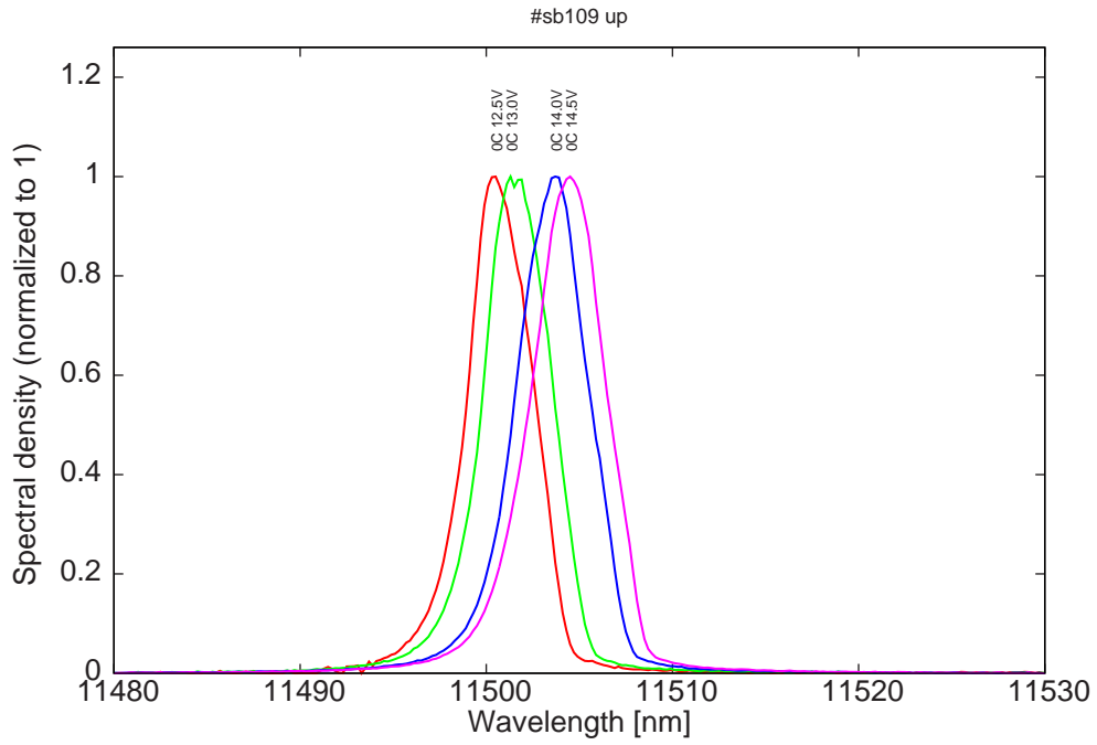
Figure 11: spectra at 0C at 2% dc for various LDD voltages
