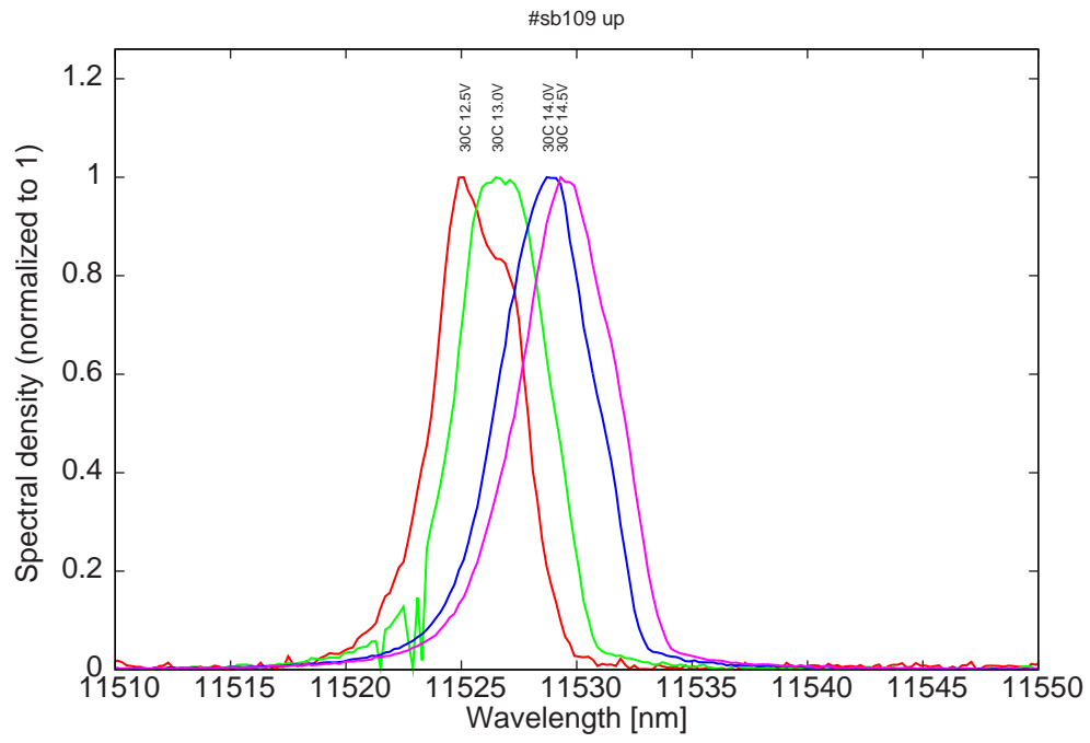
Figure 13: spectra at 30C at 2% dc for various LDD voltages
