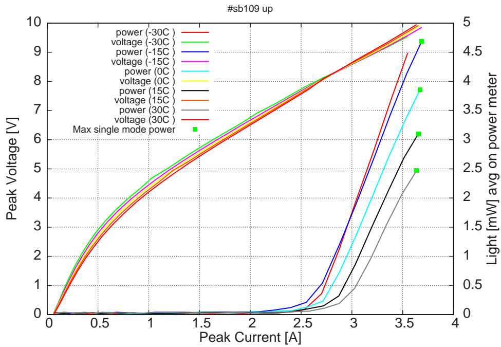
Figure 5: peak voltage and avg power vs peak current at 2% dc (including the multimode region)
