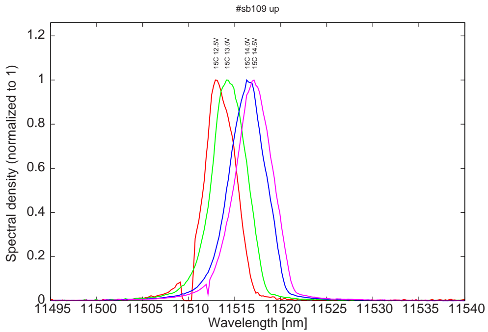
Figure 12: spectra at 15C at 2% dc for various LDD voltages
