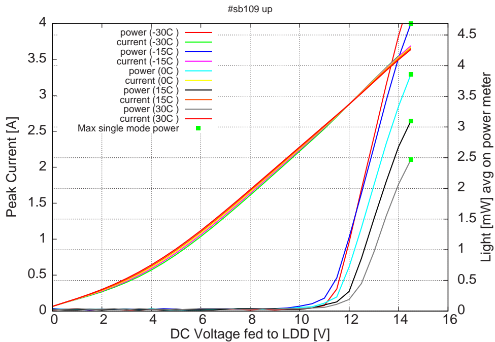
Figure 6: peak current and avg power vs LDD voltage at 2% dc (the solid squares indicate the maximum singlemode emitted power)
