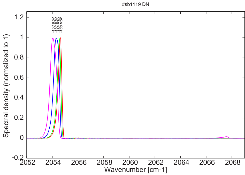
Figure 10: spectra at -15C for various LDD voltages (monomode up to 8.5V)
