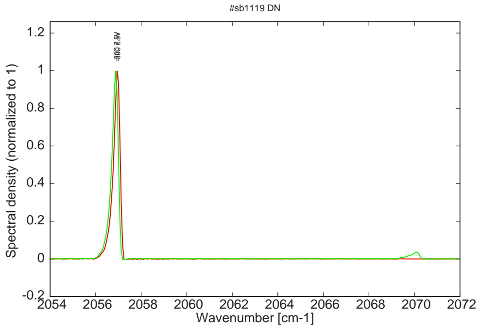
Figure 8: spectra at -30C for various LDD voltages (monomode only at threshold)
