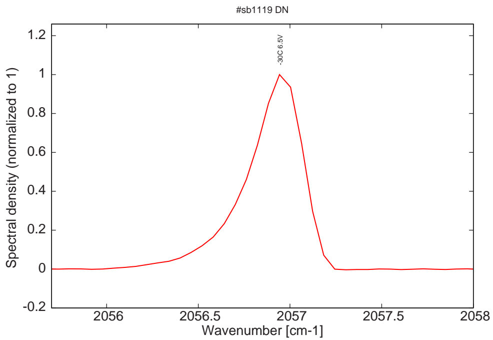
Figure 9: monomode spectrum at -30C and 6.5V
