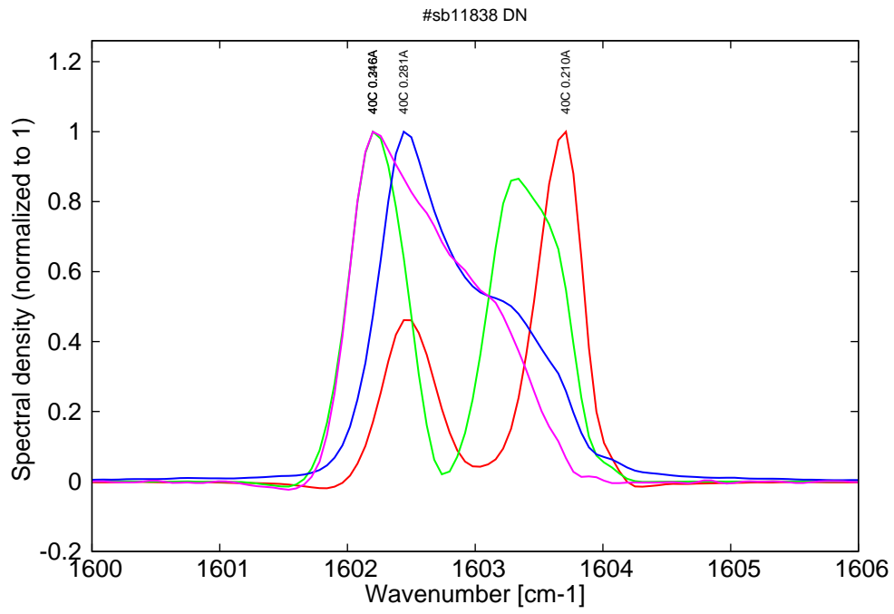
Figure 5: spectra at 40C for various peak currents at 2% duty-cycle (500ns pulses on the laser)
