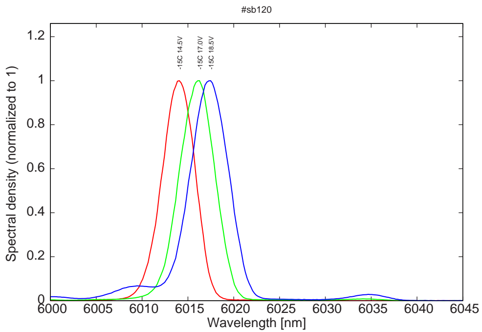
Figure 10: spectra at -15C for various LDD voltages (monomode only up to 15V)
