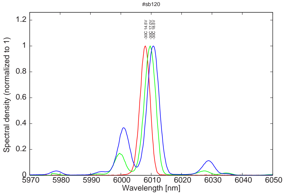
Figure 9: spectra at -30C for various LDD voltages (monomode only up to 14.5V)
