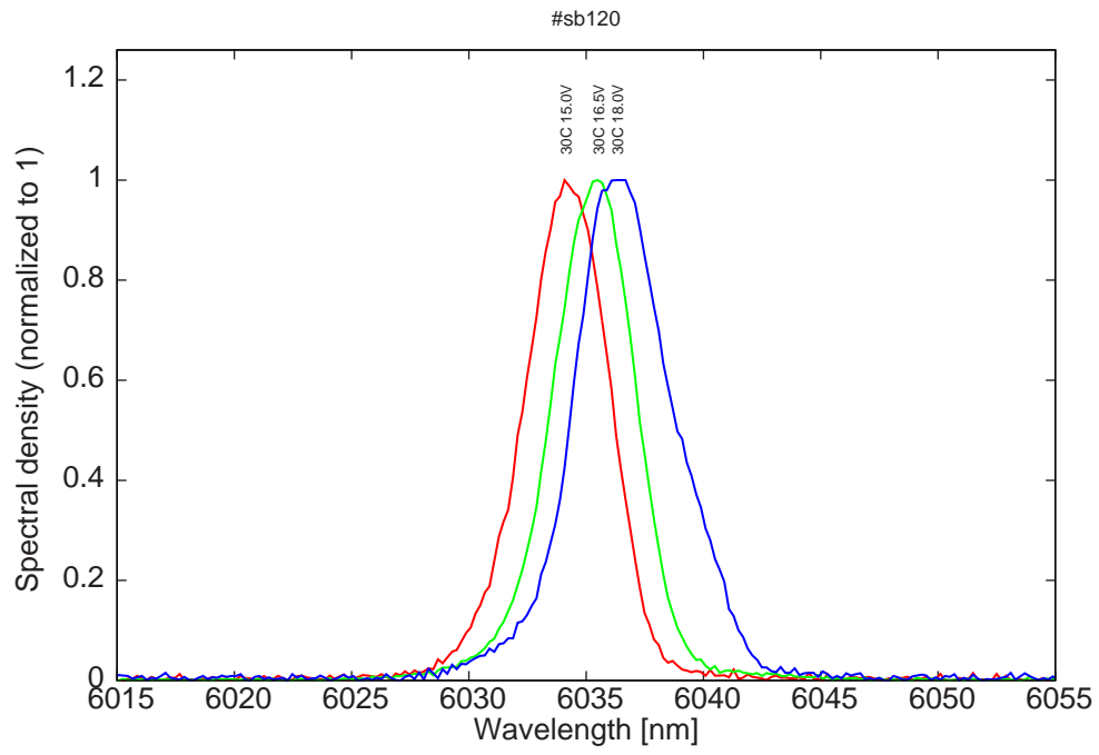
Figure 13: spectra at 30C for various LDD voltages (monomode)
