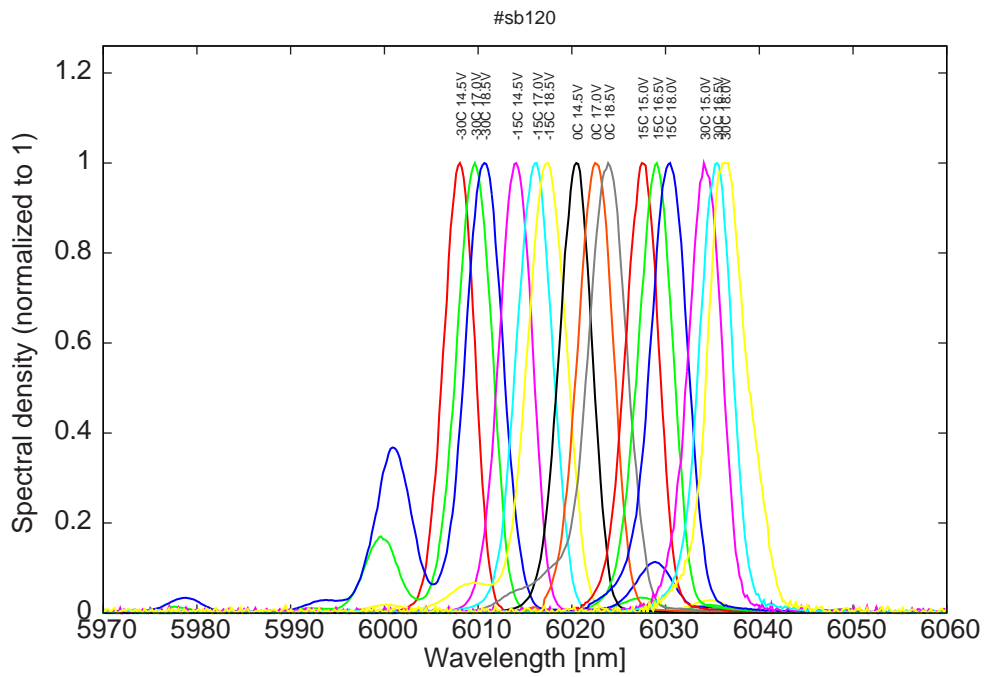
Figure 8: spectra at -30C, -15C, 0C, 15C, and 30C for various LDD voltages
