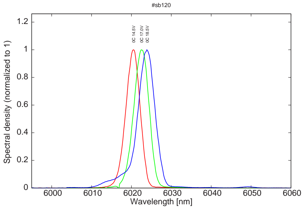
Figure 11: spectra at 0C for various LDD voltages (monomode only up to 16.5V)
