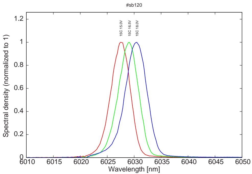
Figure 12: spectra at 15C for various LDD voltages (monomode)
