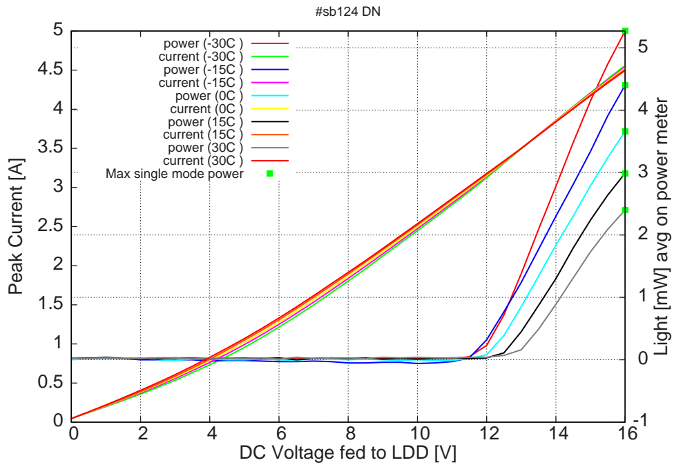
Figure 5: peak current and avg power vs LDD voltage at 2% dc (the solid squares indicate the maximum singlemode emitted power)
