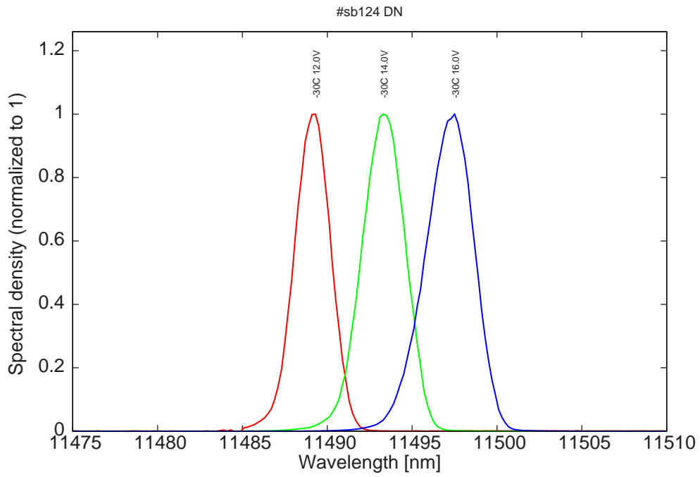
Figure 7: spectra at -30C at 2% dc for various LDD voltages
