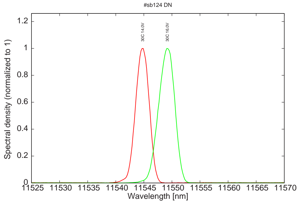
Figure 11: spectra at 30C at 2% dc for various LDD voltages
