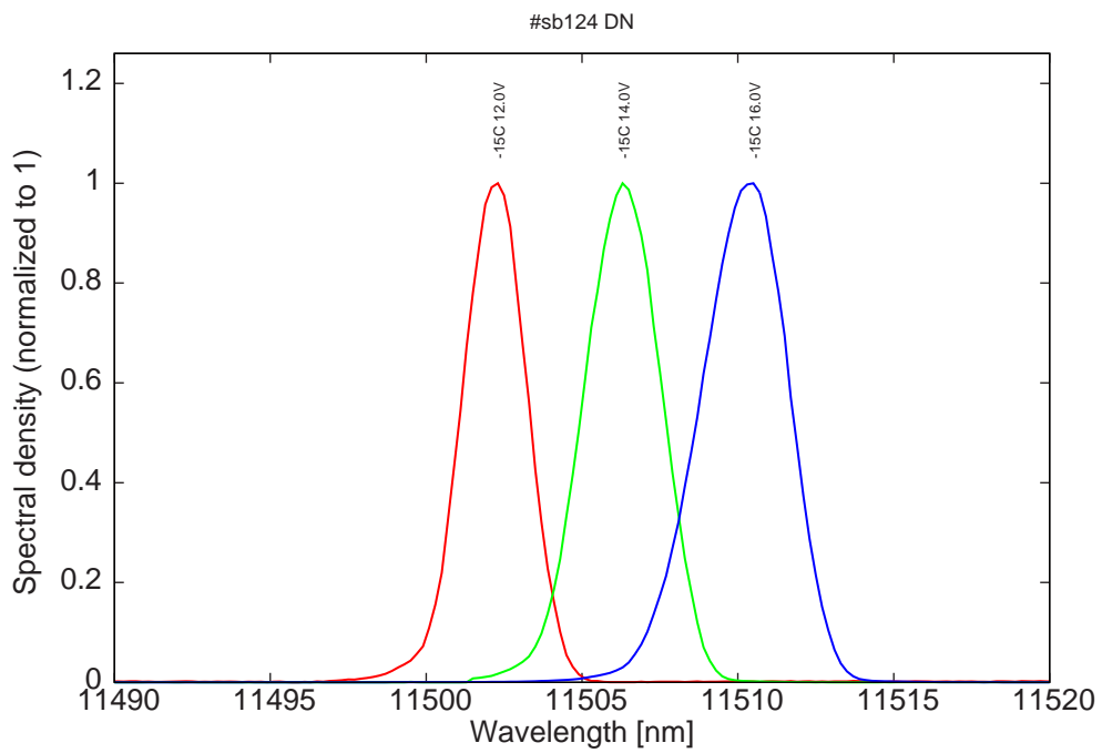
Figure 8: spectra at -15C at 2% dc for various LDD voltages
