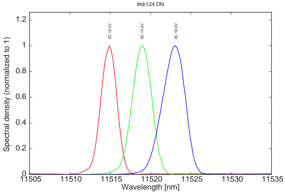
Figure 9: spectra at 0C at 2% dc for various LDD voltages
