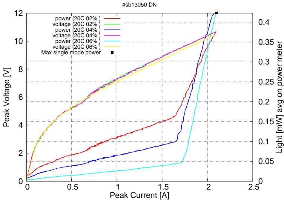
Figure 6: Peak voltage and average power vs peak current at 20C for various duty-cycle (200ns pulses on the laser) (the solid squares indicate the maximum singlemode emitted power)
