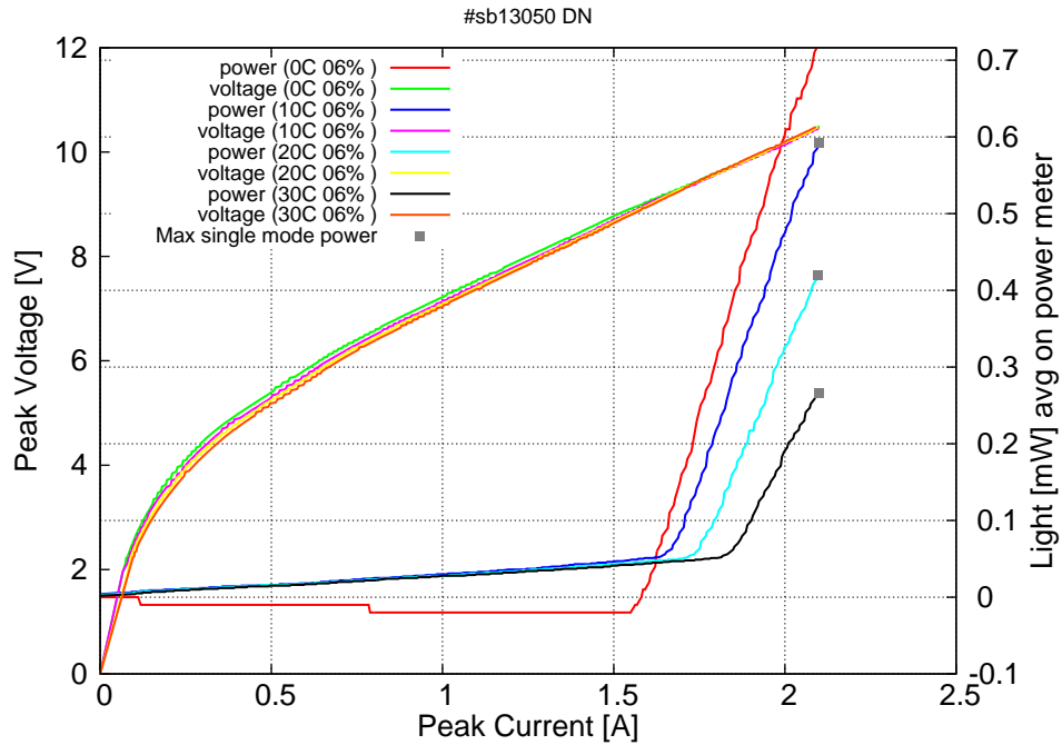
Figure 4: Peak voltage and average power vs peak current at 6% duty-cycle (200ns pulses on the laser) (the solid squares indicate the maximum singlemode emitted power)
