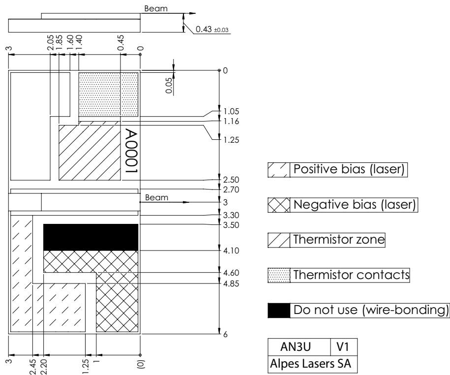
Figure 1: Mechanical and electrical interface for #sb13188 DN (please note that AlN submount numbering is A08TV)
