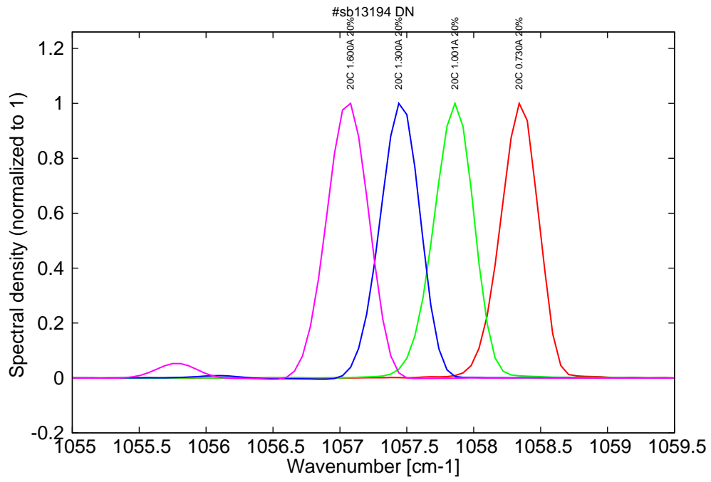
Figure 7: spectra at 20C and 20% duty-cycle (100ns pulses on the laser). monomode up to 1A, then becomes bimode
