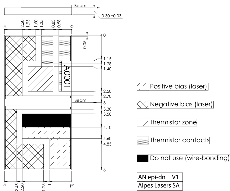
Figure 1: Mechanical and electrical interface for #sb13194 DN (please note that AlN submount numbering is A02AH)
