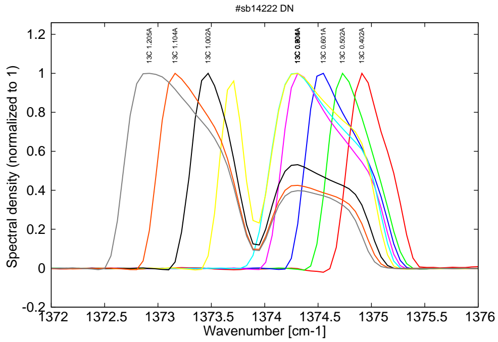
Figure 5: spectra at ^{13}\text{C} for various peak currents at 2% duty cycle (500ns pulses on the laser)
