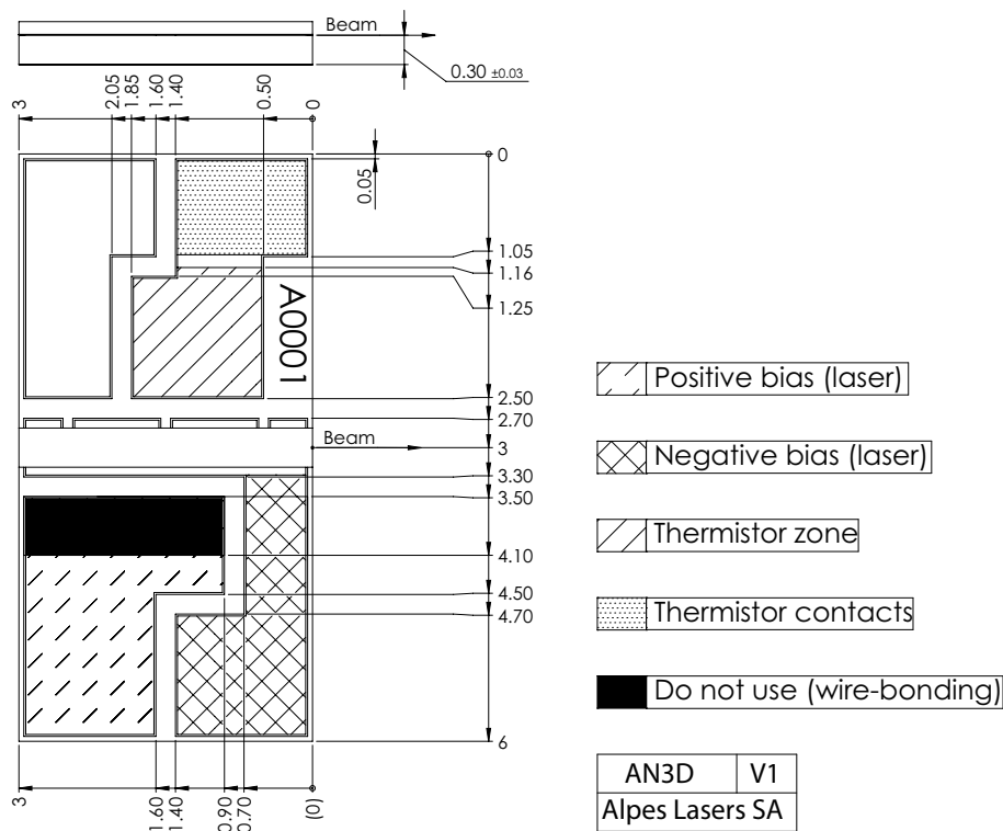
Figure 1: Mechanical and electrical interface for #sb14222 DN (please note that AlN submount numbering is P0539)
