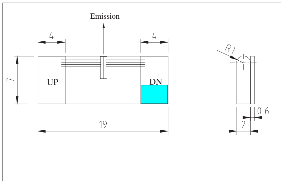
Figure 1: Support mounting for #sb152 (please note that the laser is connected to the DN pad drawn in blue)
