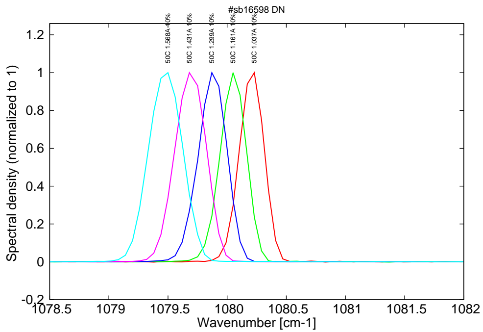
Figure 8: spectra at 50C at 10% duty-cycle (60ns pulses on the laser)
