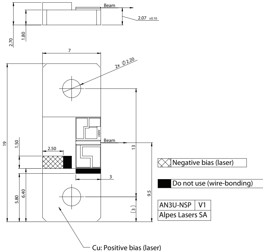
Figure 1: Mechanical and electrical interface for #sb16598 DN
