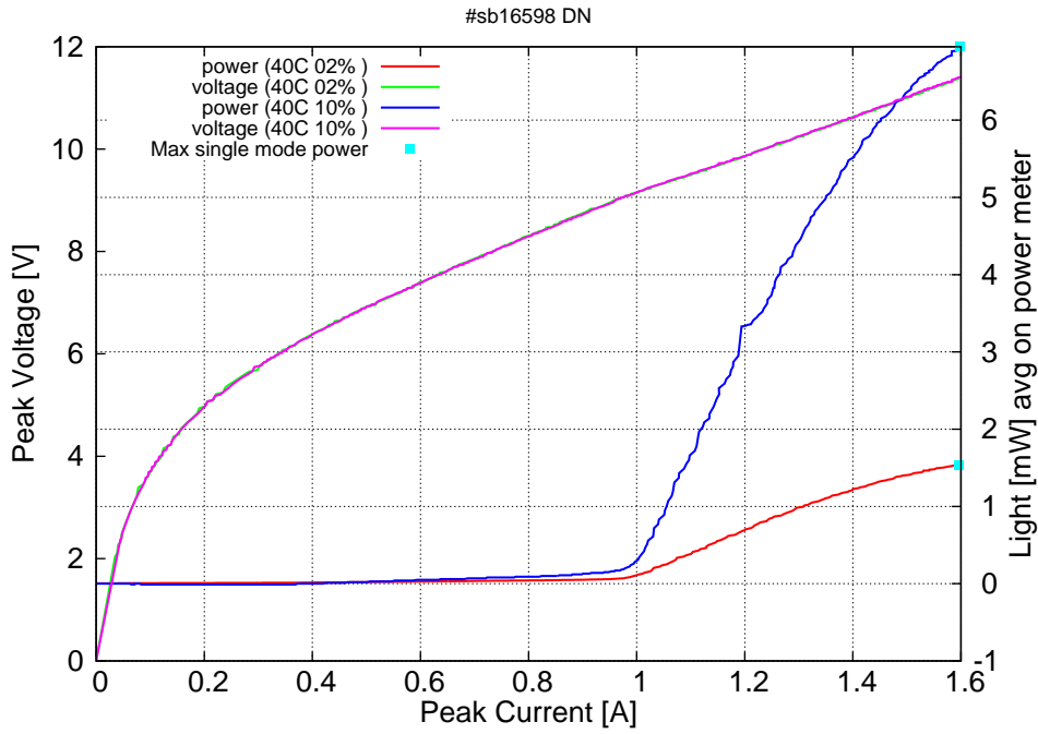
Figure 5: Peak voltage and average power vs peak current at 40C at 2% and 10% duty-cycle (500ns pulses on the laser) / I_{max}=1.60A / duty max = 10% (the solid squares indicate the maximum singlemode emitted power)
