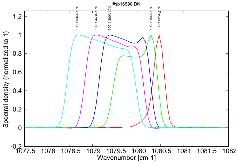
Figure 9: spectra at 50C at 10% duty-cycle with 300ns pulses on the laser
