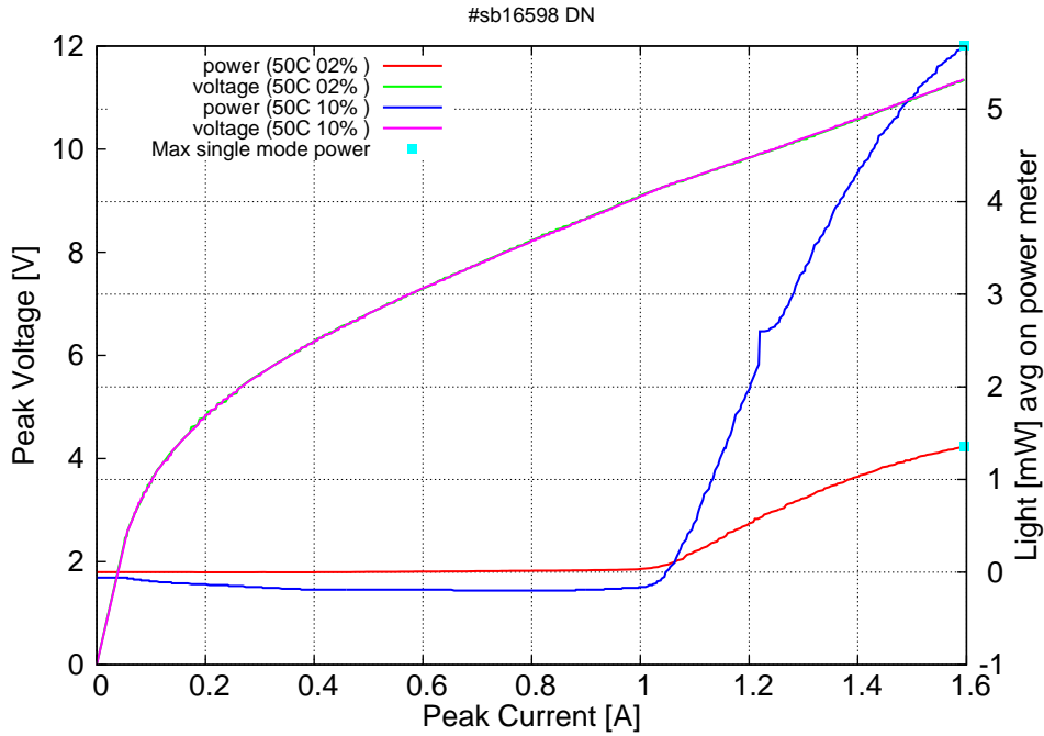
Figure 6: Peak voltage and average power vs peak current at 50C at 2% and 10% duty-cycle (500ns pulses on the laser) / I_{max}=1.60A / duty max = 10% (the solid squares indicate the maximum singlemode emitted power)
