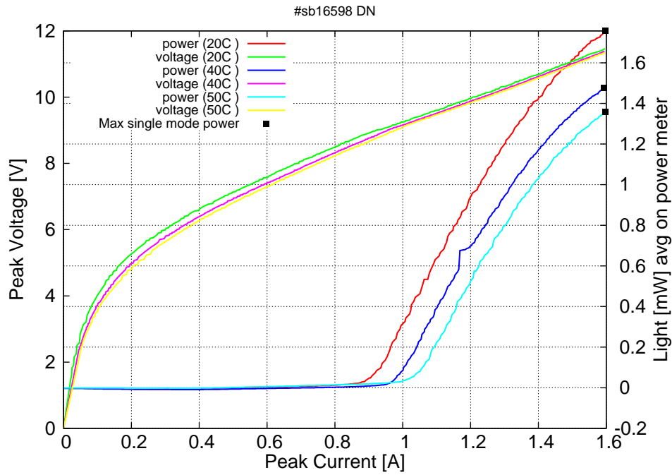
Figure 4: Peak voltage and average power vs peak current at 2% duty-cycle (500ns pulses on the laser) / I_{max}=1.60A (the solid squares indicate the maximum singlemode emitted power)
