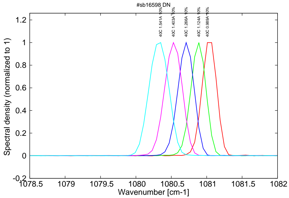
Figure 7: spectra at 40C at 10% duty-cycle (60ns pulses on the laser)
