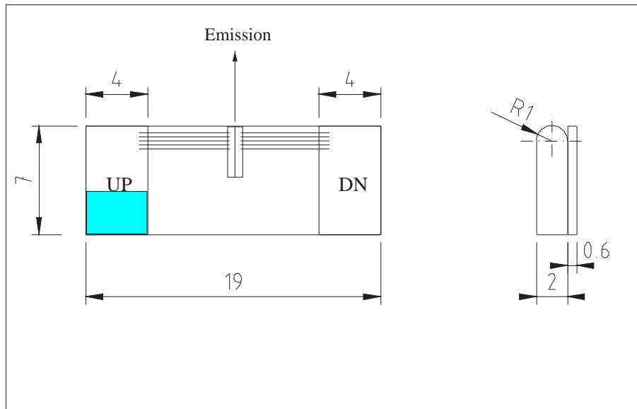
Figure 1: Support mounting for #sb170 (please note that the laser is connected to the UP pad drawn in blue)
