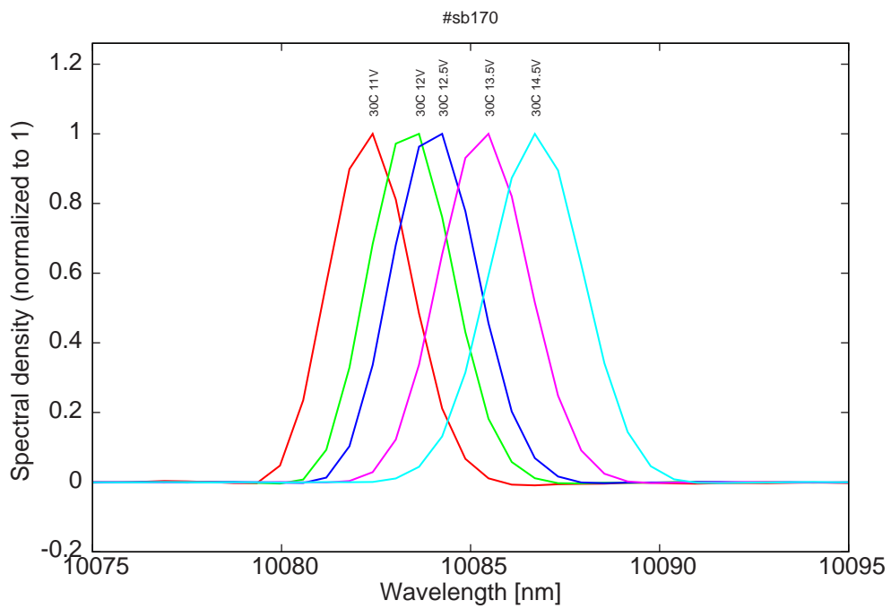
Figure 14: spectra at 30C for various LDD voltages
