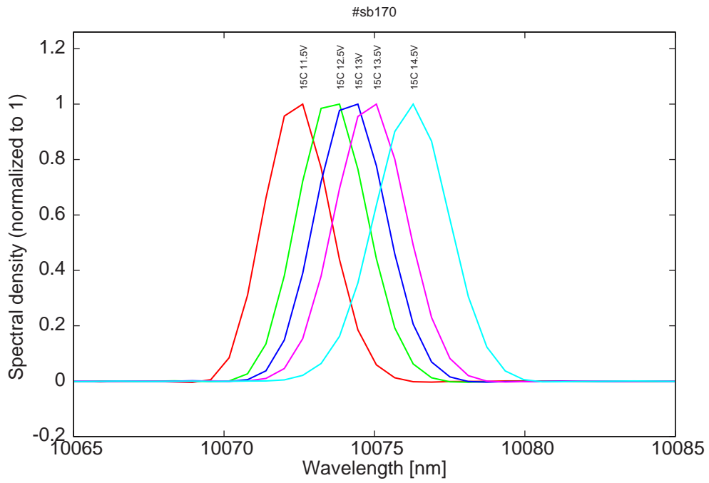
Figure 13: spectra at 15C for various LDD voltages
