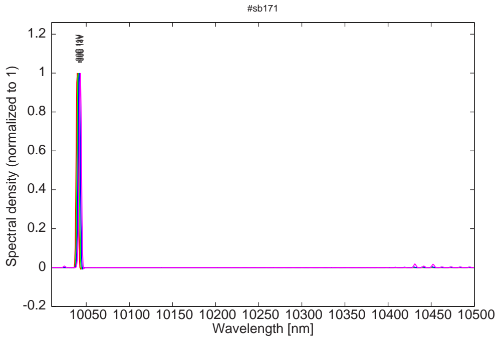
Figure 9: spectra at -30C for various LDD voltages
