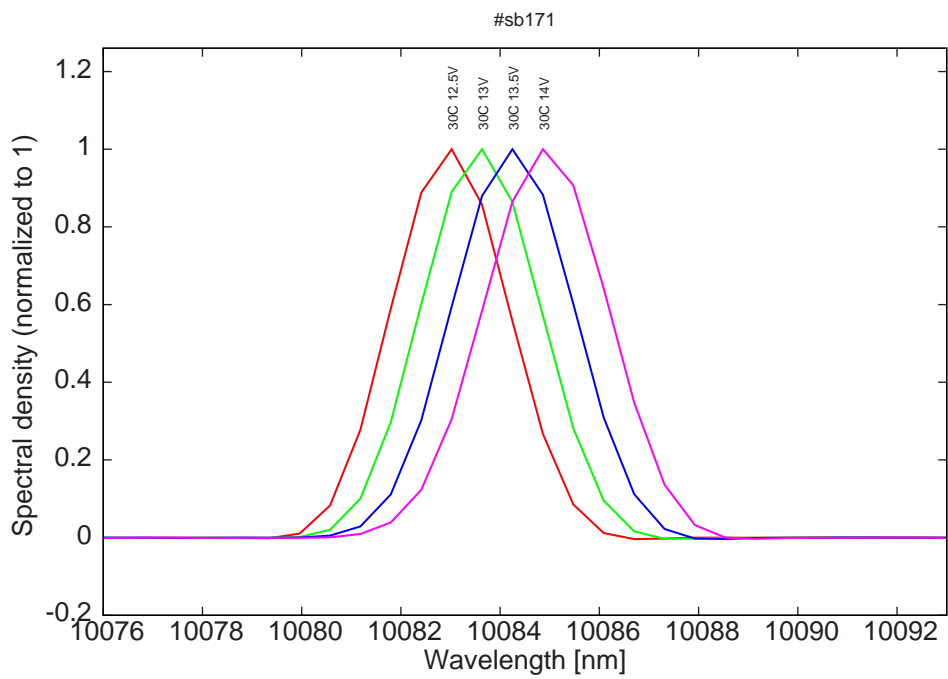
Figure 16: spectra at 30C for various LDD voltages
