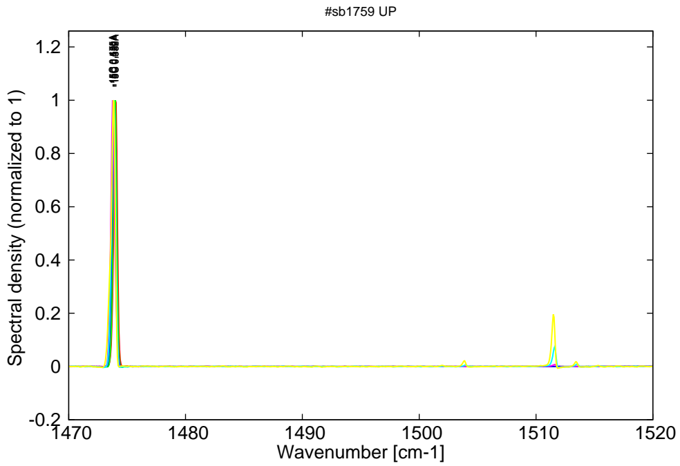
Figure 8: spectra at -15C for various DC currents (monomode up to 0.420A, then becomes multi)
