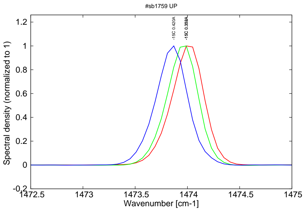
Figure 9: spectra at -15C for various DC currents (monomode range)
