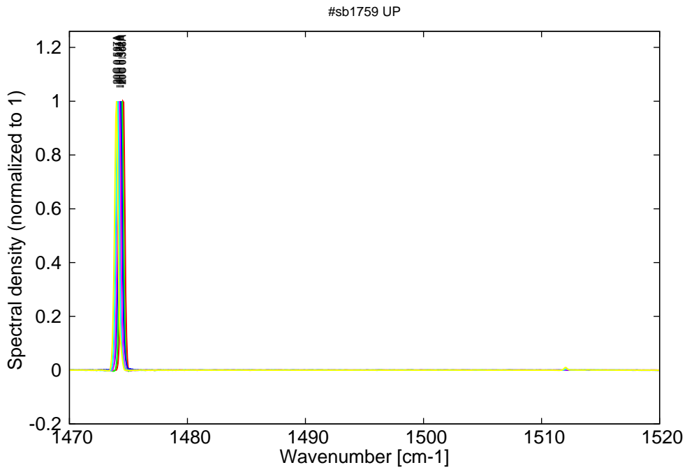
Figure 6: spectra at -20C for various DC currents (monomode up to 0.420A, then becomes multi)
