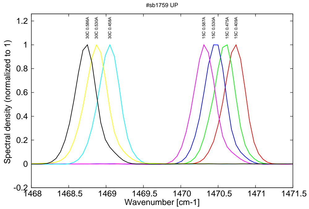
Figure 12: spectra at 15C and 30C for various DC currents (all monomode)
