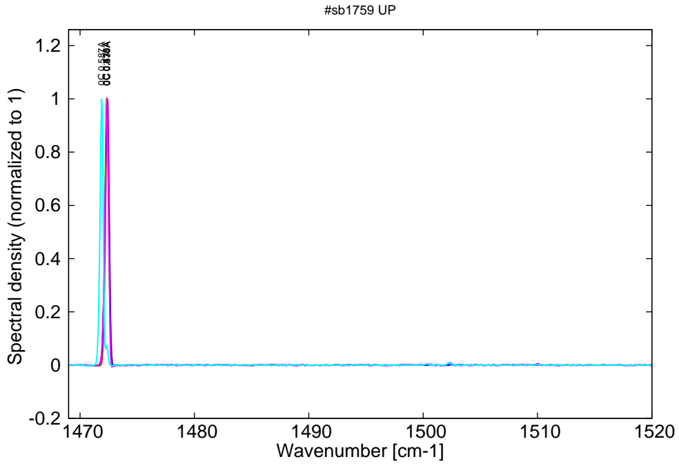
Figure 10: spectra at 0C for various DC currents (monomode up to 0.475A, then becomes multi)
