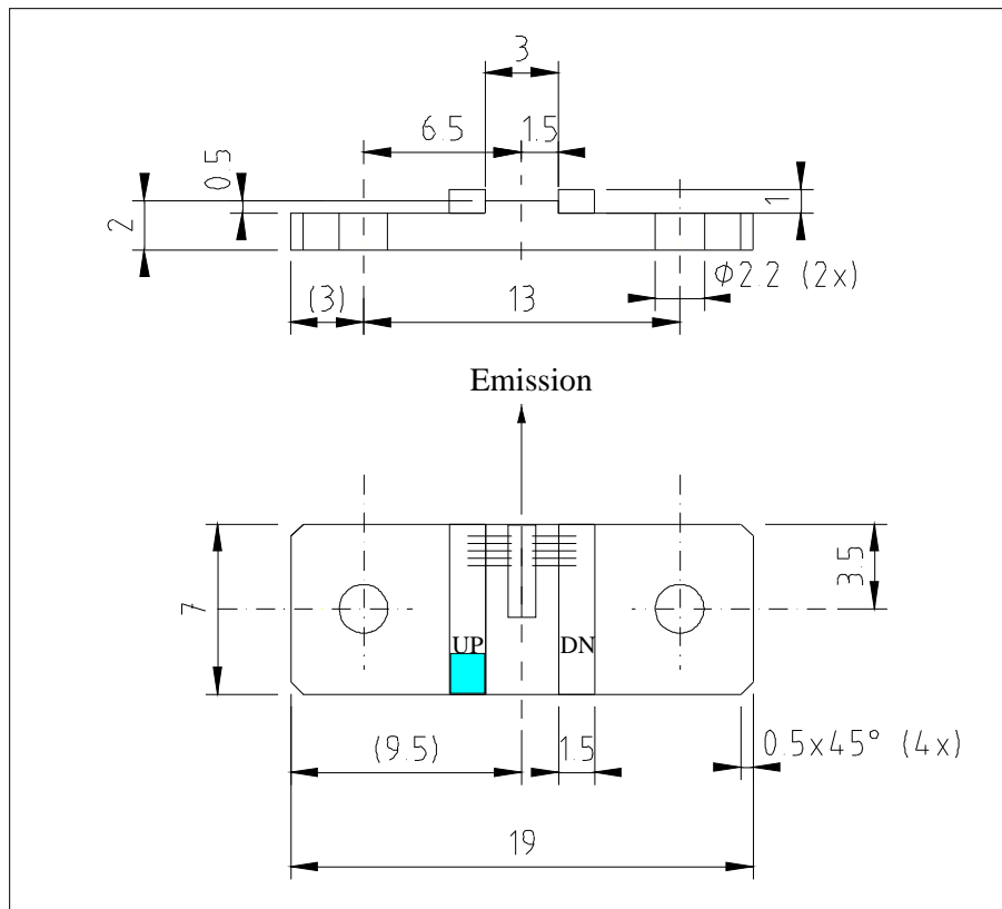
Figure 1: Support mounting for #sb1759 UP (please note that the laser is connected to the UP pad drawn in blue)
