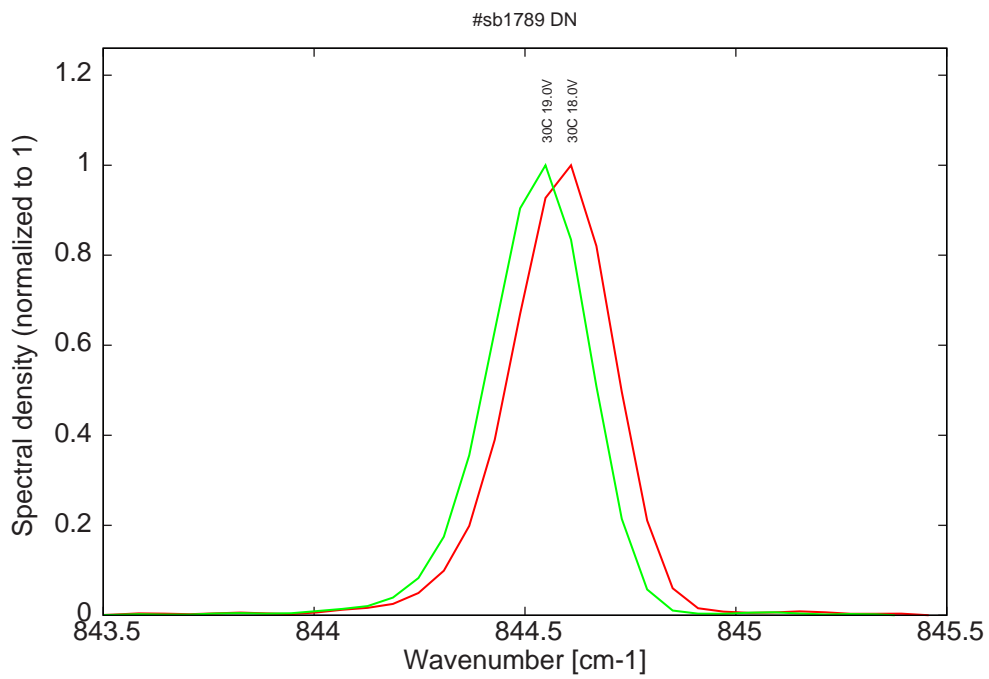
Figure 17: spectra at 30C for various LDD voltages (monomode range)
