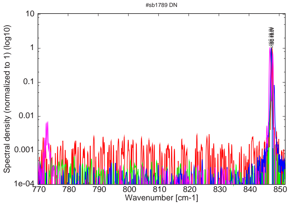
Figure 10: spectra at -15C for various LDD voltages (modes around 773cm-1)
