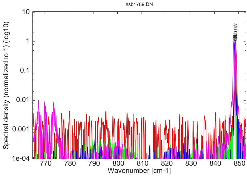
Figure 8: spectra at -30C for various LDD voltages (modes around 770cm-1)
