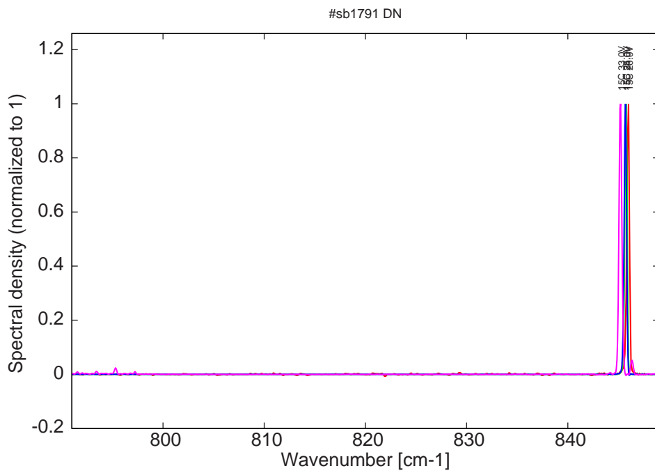
Figure 13: spectra at 15C for various LDD voltages
