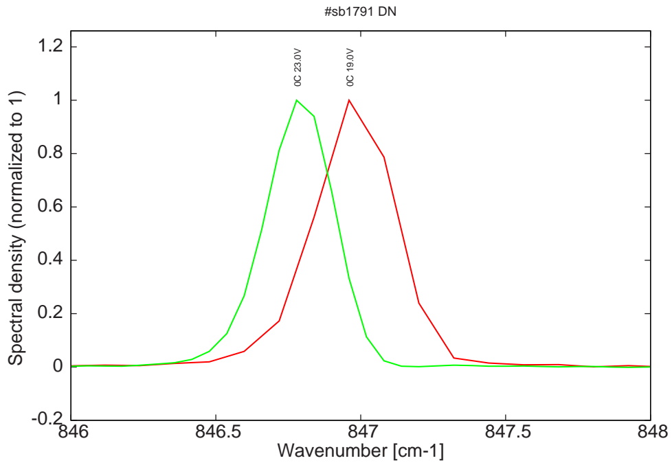
Figure 12: spectra at 0C for various LDD voltages ( monomode range)
