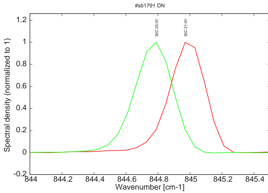
Figure 16: spectra at 30C for various LDD voltages ( monomode range)
