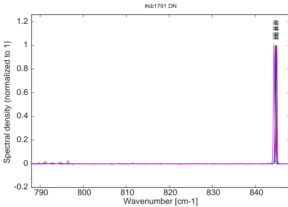
Figure 15: spectra at 30C for various LDD voltages
