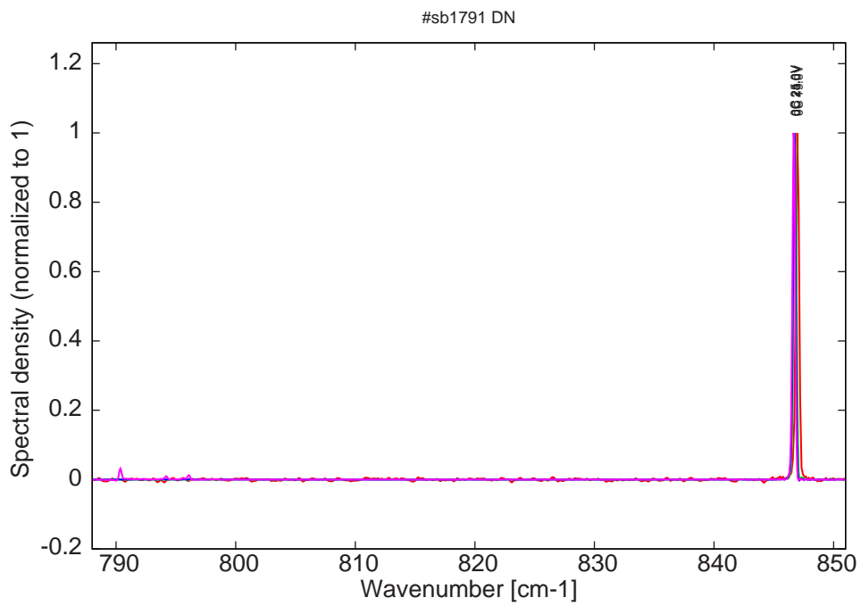
Figure 11: spectra at 0C for various LDD voltages
