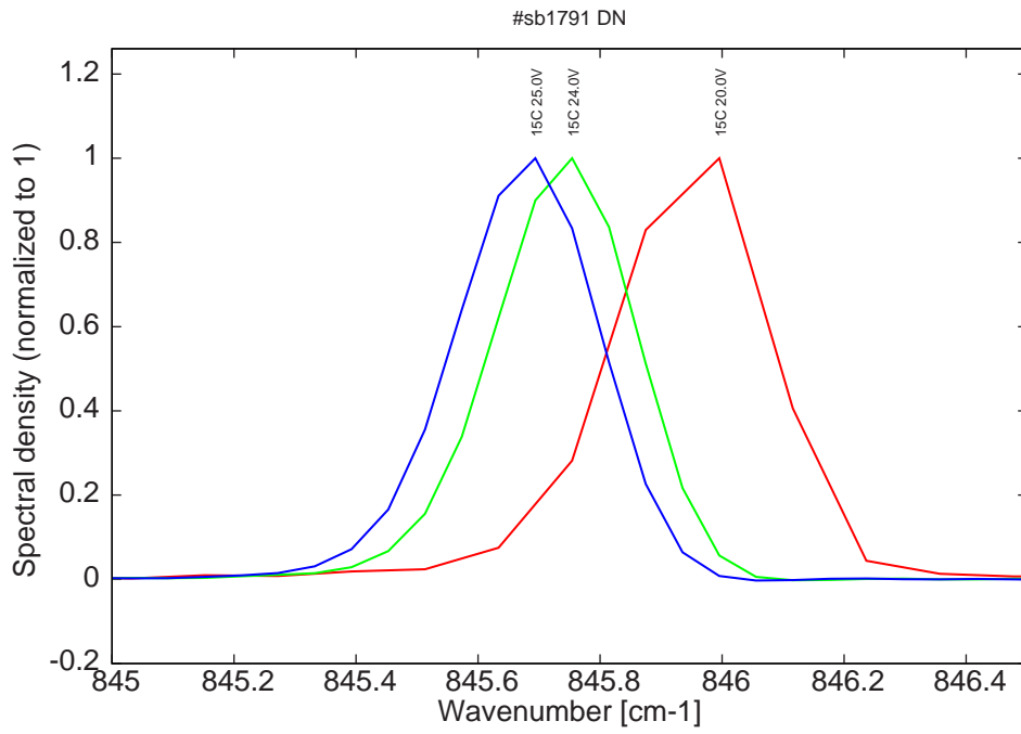
Figure 14: spectra at 15C for various LDD voltages ( monomode range)
