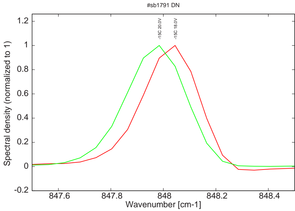
Figure 10: spectra at -15C for various LDD voltages ( monomode range)
