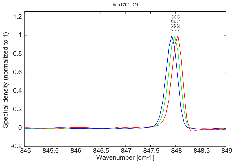
Figure 9: spectra at -15C for various LDD voltages (small mode around 845.6cm-1 at 21V on LDD )
