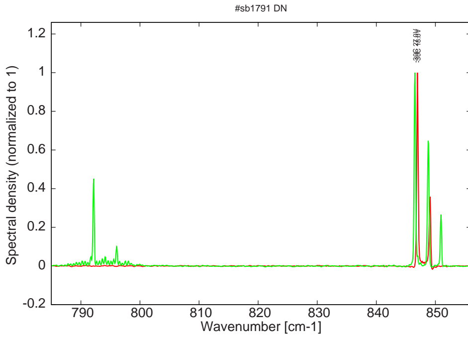
Figure 8: spectra at -30C for various LDD voltages
