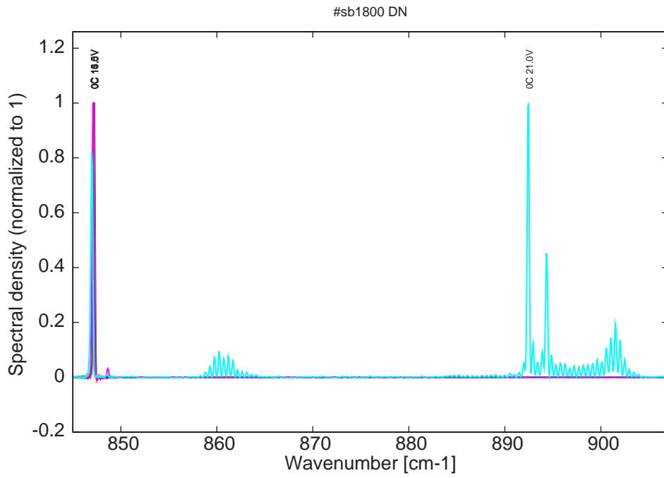
Figure 12: spectra at 0C for various LDD voltages
