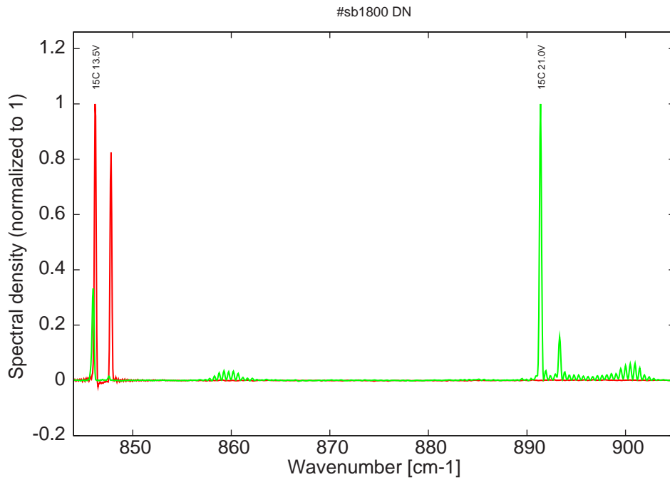
Figure 14: spectra at 15C for various LDD voltages (all bi- or multimode)
