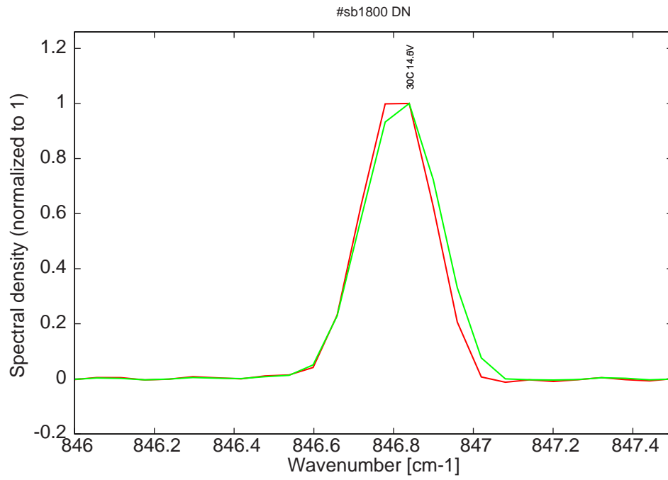
Figure 16: spectra at 30C for various LDD voltages (monomode range, but with mode jumping compared to spectra at 0C, see Fig. 1)
