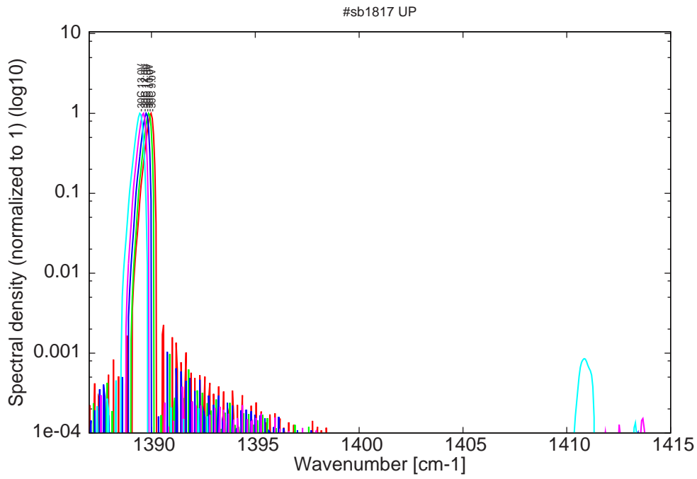
Figure 8: spectra at -30C for various LDD voltages; monomode up to 12V (22ns pulses, 1.1 \mu s period)
