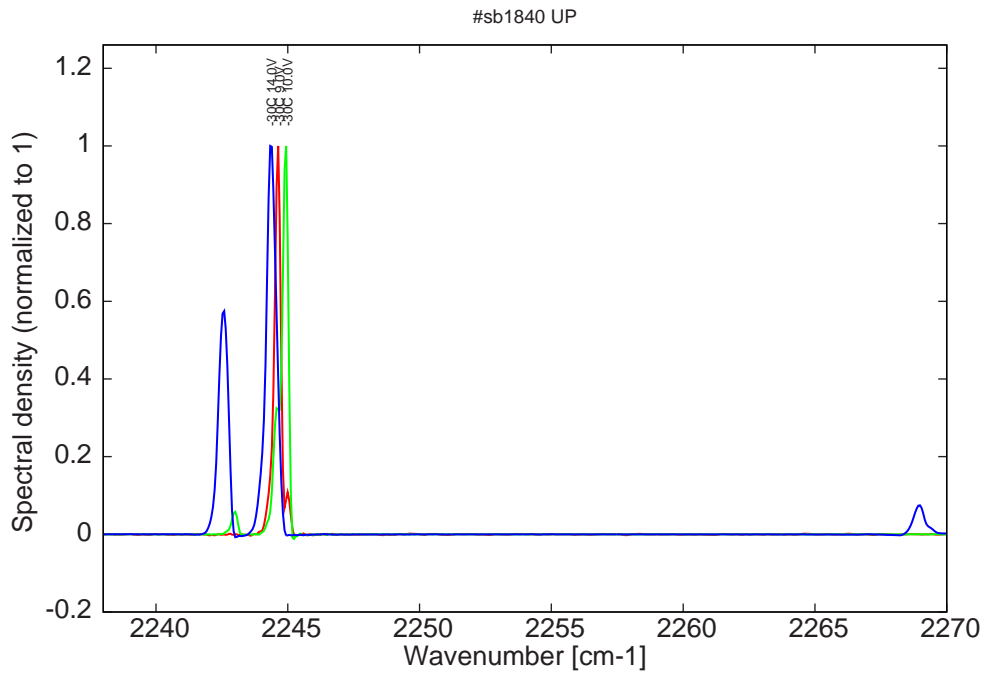
Figure 8: spectra at -30C for various LDD voltages at 2% duty-cycle (22ns pulses on the laser, 1.1 \mu s period); all multimode
