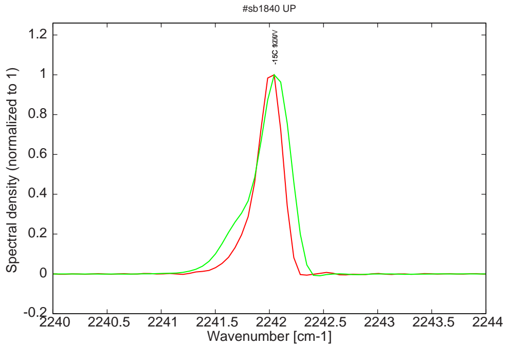
Figure 10: spectra at -15C for various LDD voltages at 2% duty-cycle (monomode range)
