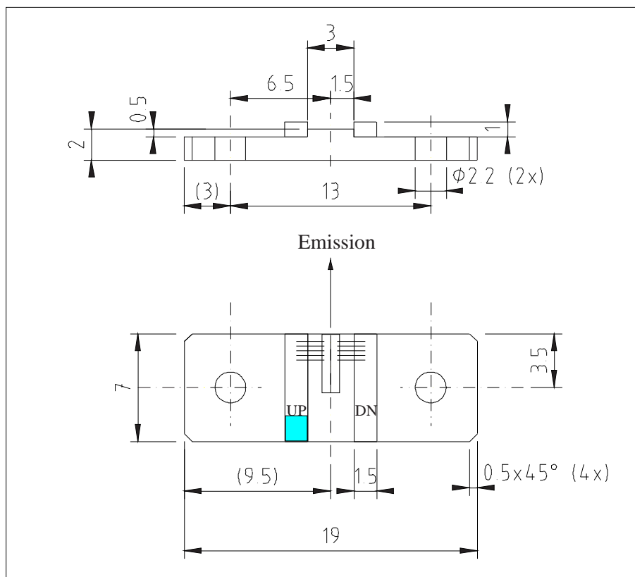
Figure 1: Support mounting for #sb1840 UP (please note that the laser is connected to the UP pad drawn in blue)
