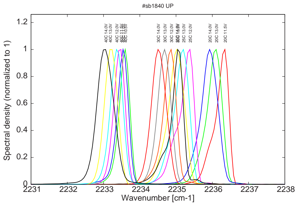
Figure 15: spectra between 20C and 40C for various LDD voltages at 2% duty-cycle (22ns pulses on the laser, 1.1 \mu s period); all monomode
