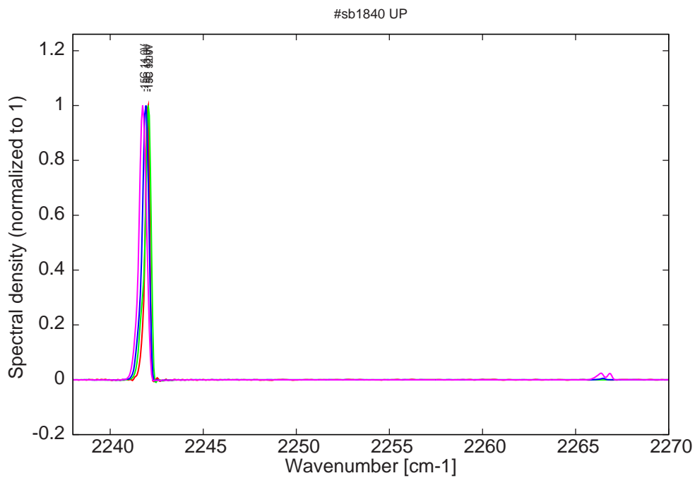
Figure 9: spectra at -15C for various LDD voltages at 2% duty-cycle (22ns pulses on the laser, 1.1 \mu s period)
