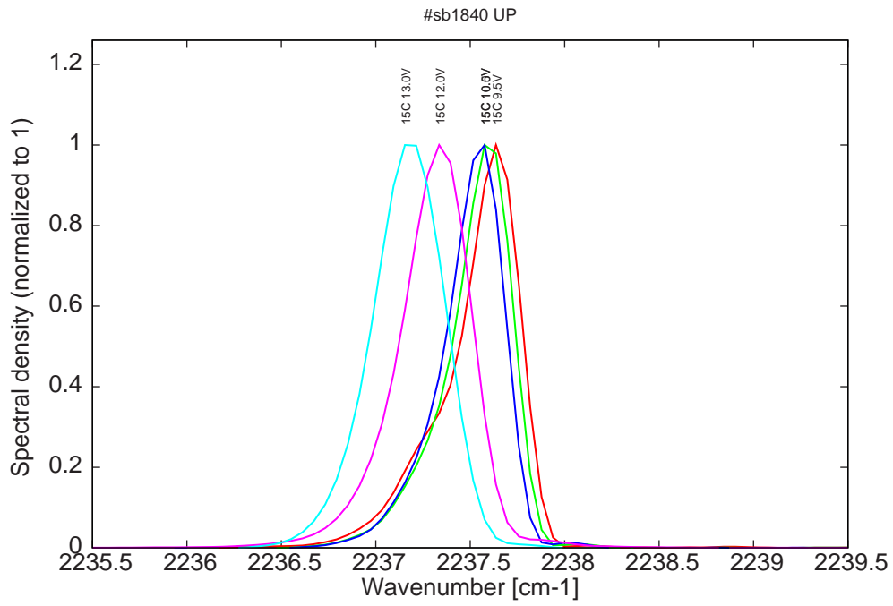
Figure 14: spectra at 15C for various LDD voltages at 2% duty-cycle (monomode range)
