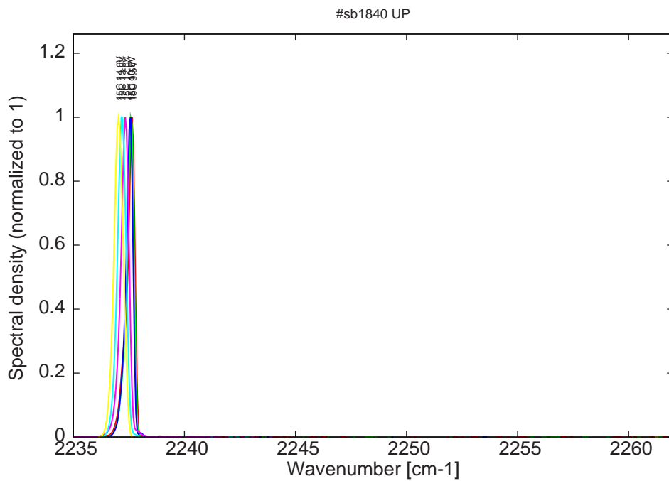
Figure 13: spectra at 15C for various LDD voltages at 2% duty-cycle (22ns pulses on the laser, 1.1 \mu s period); small mode around 2260cm-1 at 14.0V on LDD
