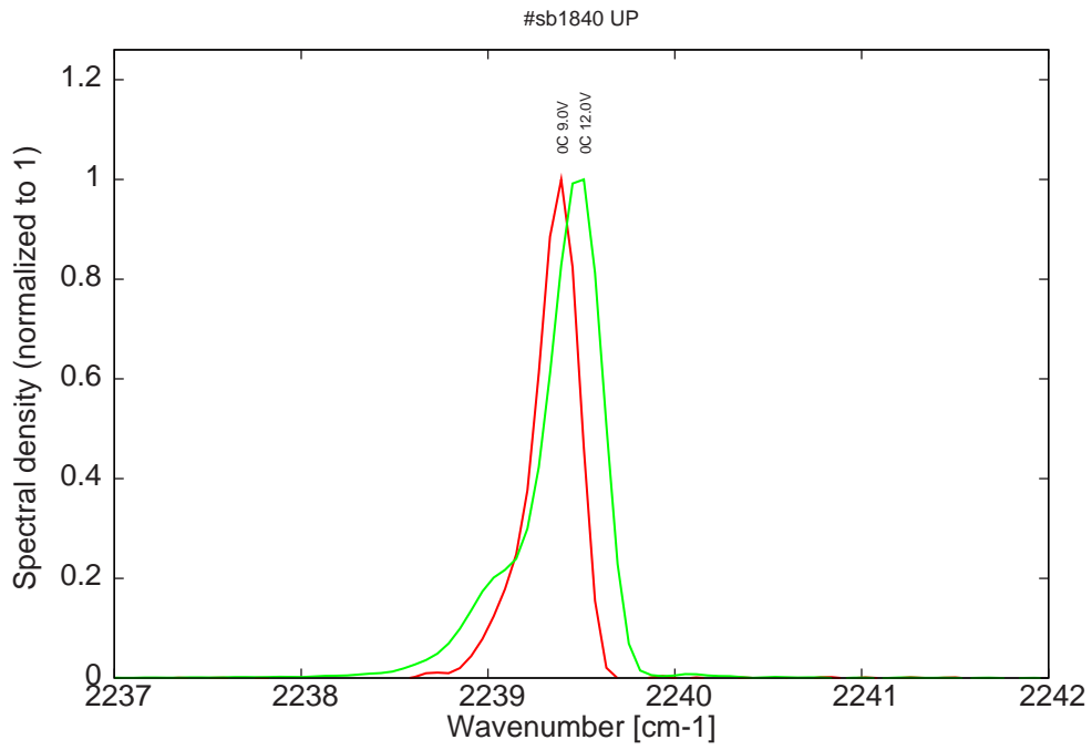
Figure 12: spectra at 0C for various LDD voltages at 2% duty-cycle (monomode range)
