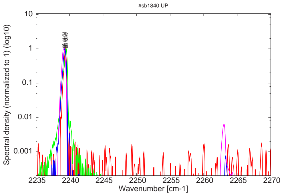
Figure 11: spectra at 0C for various LDD voltages at 2% duty-cycle (22ns pulses on the laser, 1.1 \mu s period); small modes around 2263cm-1
