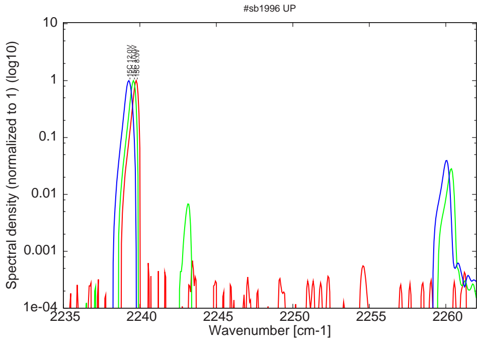
Figure 9: spectra at -15C for various LDD voltage (22ns pulses on the laser); monomode only at threshold
