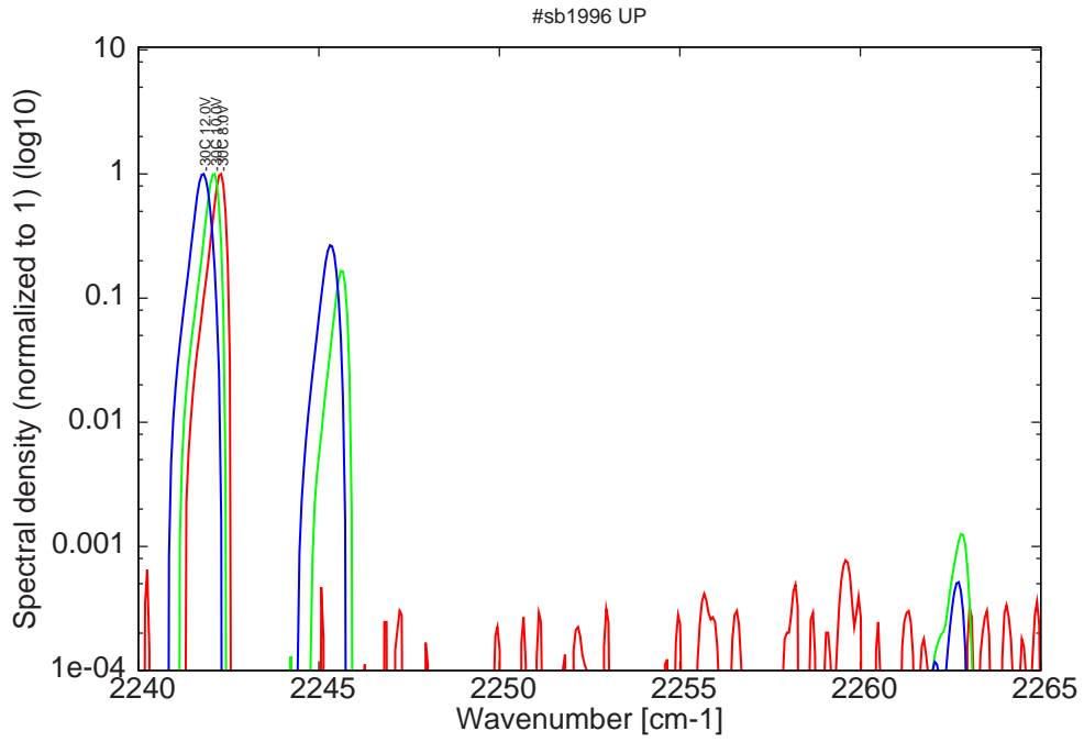
Figure 8: spectra at -30C for various LDD voltage (22ns pulses on the laser); monomode only at threshold
