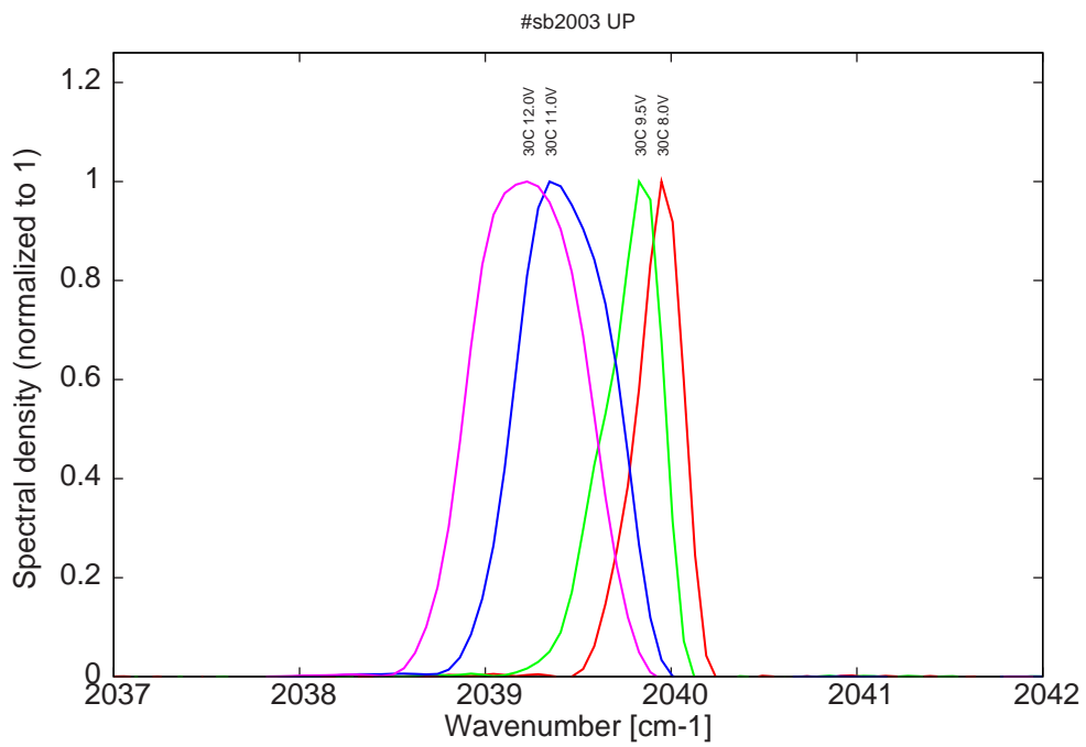
Figure 15: spectra at 30C for various LDD voltage (all monomode)
