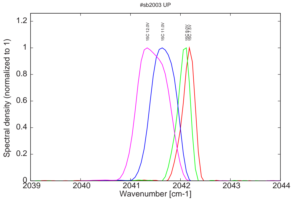
Figure 14: spectra at 15C for various LDD voltage (all monomode)
