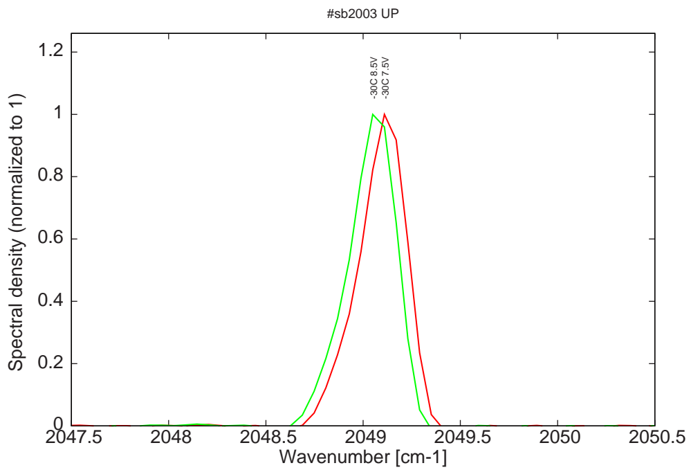
Figure 9: spectra at -30C for various LDD voltage (monomode range)
