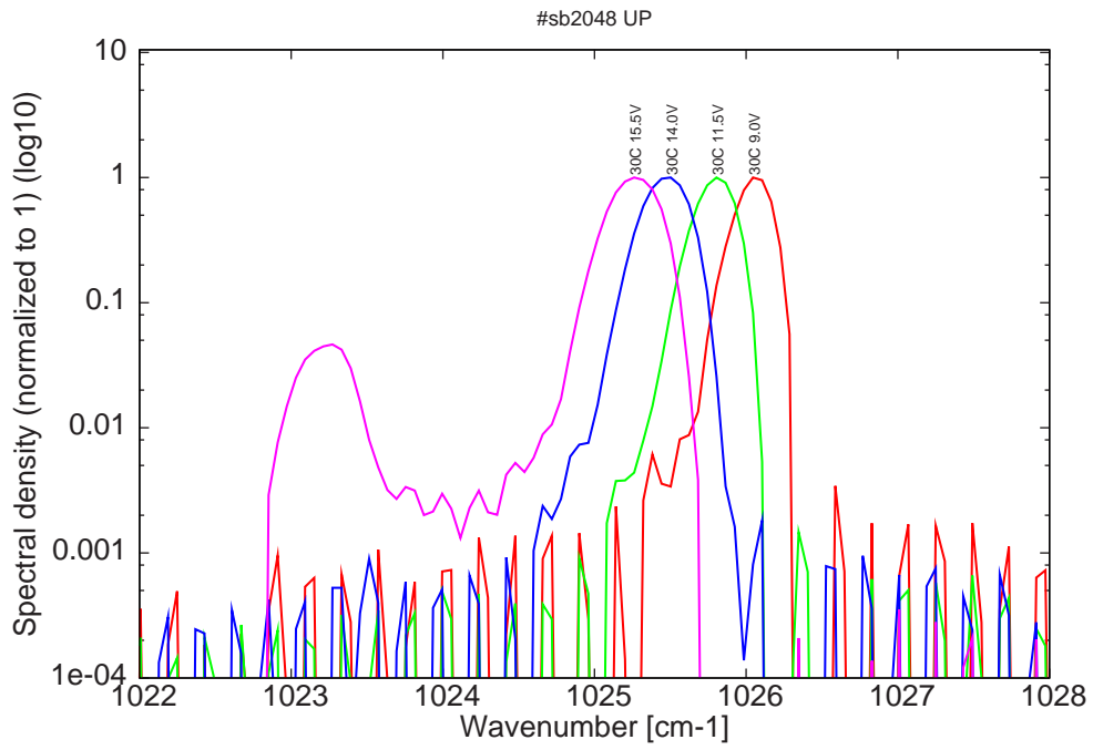
Figure 16: spectra at 30C for various LDD voltage
