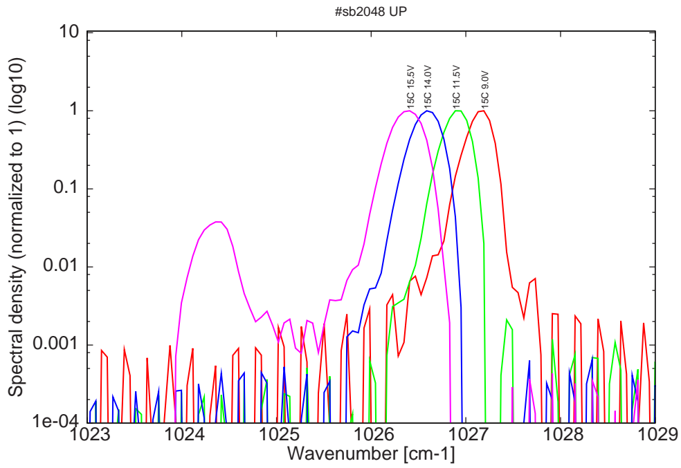
Figure 14: spectra at 15C for various LDD voltage
