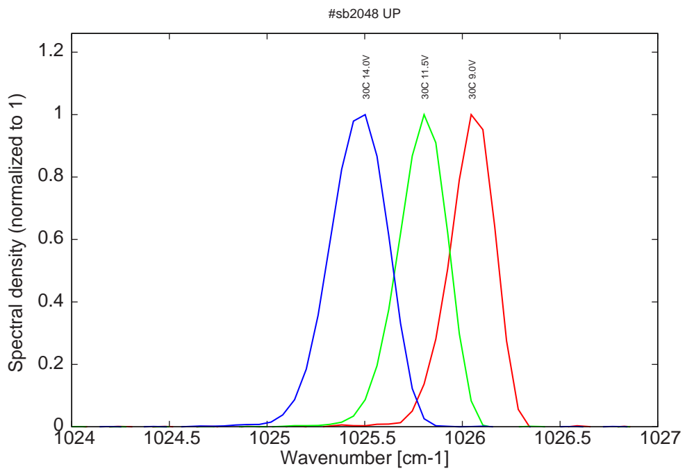
Figure 17: spectra at 30C for various LDD voltage (monomode range)
