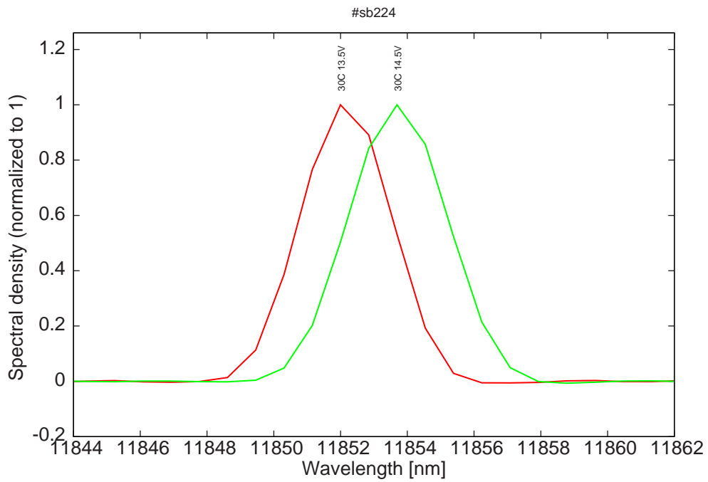
Figure 18: spectra at 30C for various LDD voltage (monomode range)
