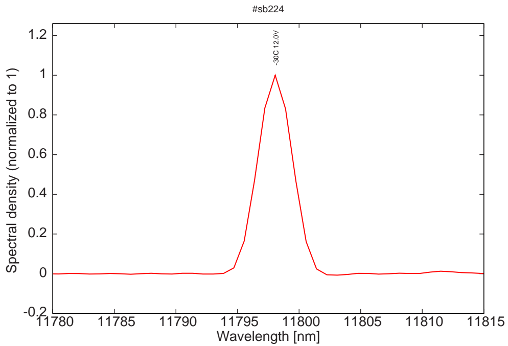
Figure 10: spectrum at -30C and 12.0V (monomode)
