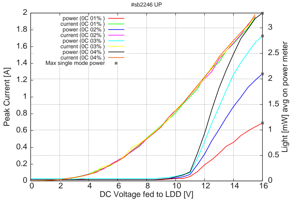
Figure 7: peak current and average power vs LDD voltage at 0C for various duty-cycles (100ns pulses on the laser) (the solid squares indicate the maximum singlemode emitted power)
