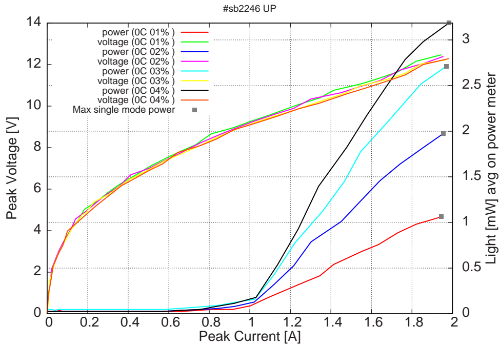
Figure 6: peak voltage and average power vs peak current at 0C for various duty-cycles (100ns pulses on the laser) (the solid squares indicate the maximum singlemode emitted power)
