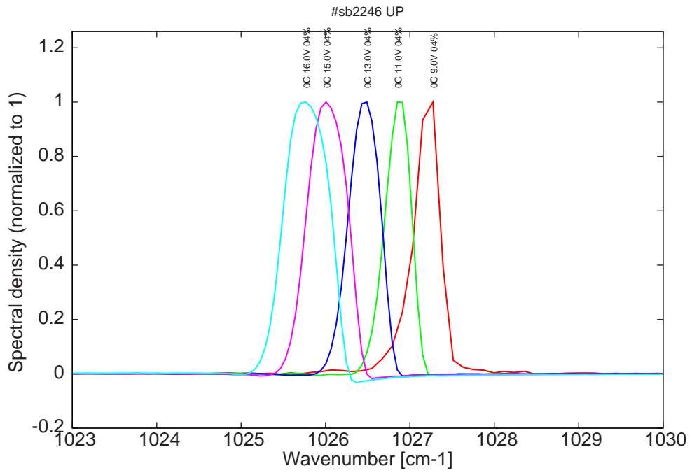
Figure 8: spectra at 0C at 4% duty-cycle for various LDD voltages (all monomode)
