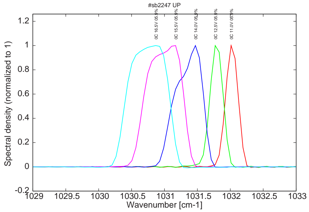
Figure 8: spectra at 0C at 6% duty-cycle for various LDD voltages (all monomode)
