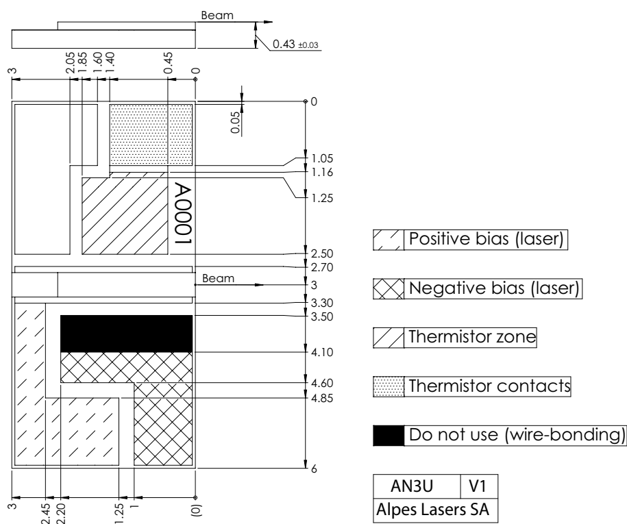
Figure 1: Mechanical and electrical interface for #sb25896 DN (please note that AlN submount numbering is A0WGW)
