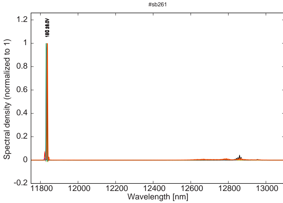
Figure 15: spectra at 15C for various LDD voltage (bimode around 11830 for voltages < 21 V)
