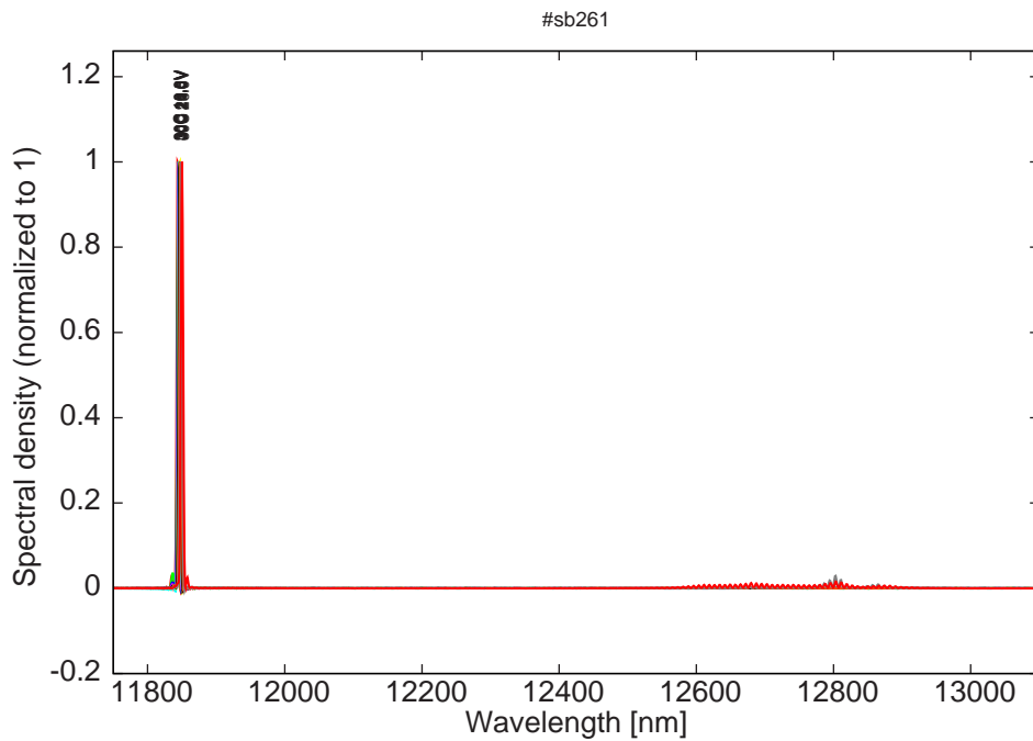
Figure 16: spectra at 30C for various LDD voltage (bimode around 11840 for voltages < 21 V)
