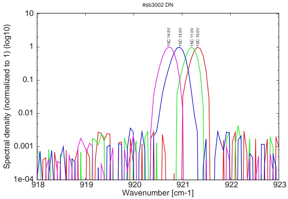
Figure 8: spectra at 15C for various LDD voltages (monomode up to 13.0V on LDD)
