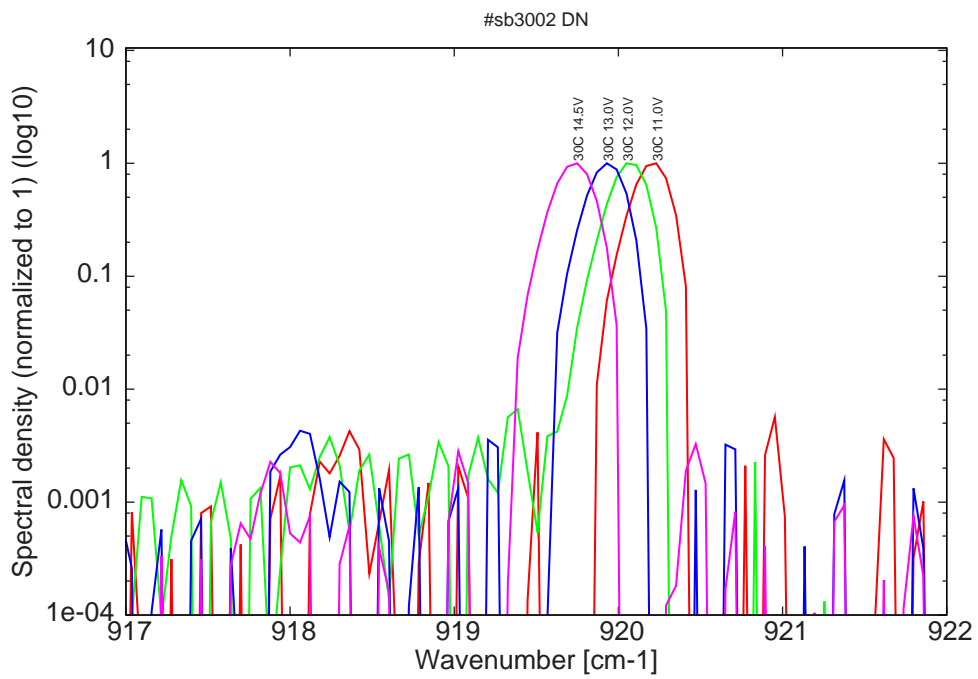
Figure 9: spectra at 30C for various LDD voltages (monomode up to 12.0V on LDD)
