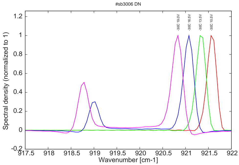
Figure 8: spectra at -30C for various LDD voltages (monomode up to 13.5V on LDD)
