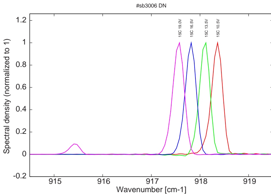
Figure 11: spectra at 15C for various LDD voltages (monomode up to 16.5V on LDD)
