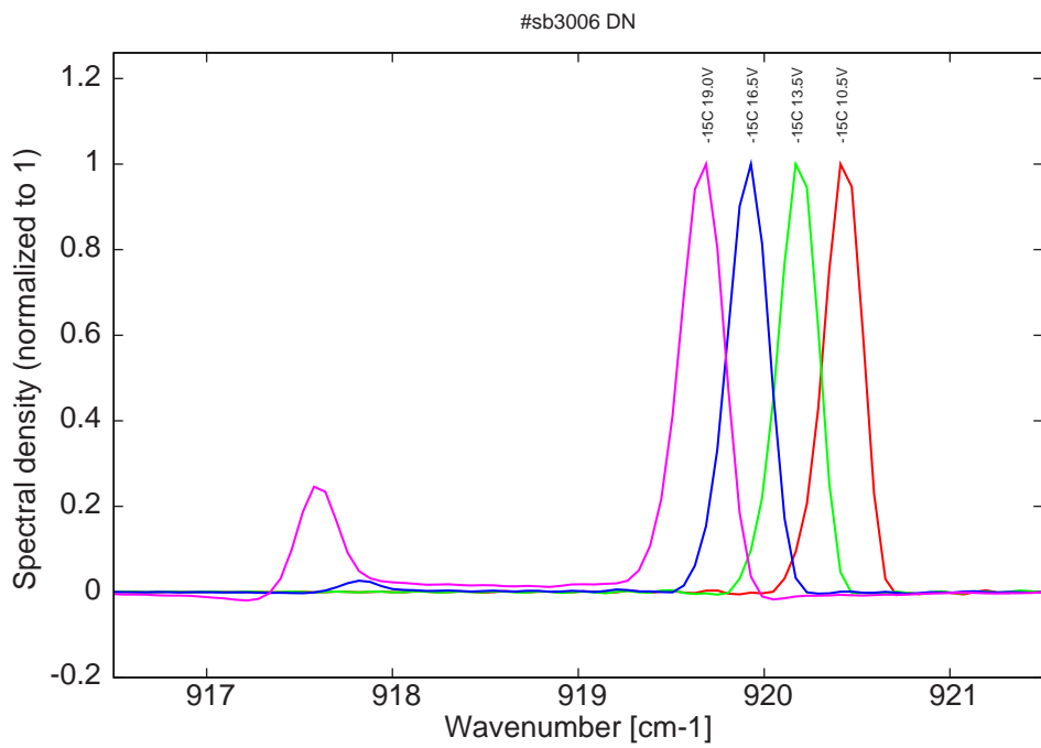
Figure 9: spectra at -15C for various LDD voltages (monomode up to 13.5V on LDD)
