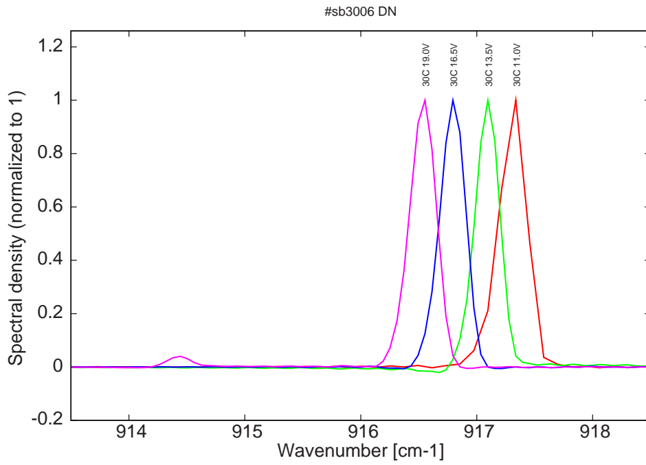
Figure 12: spectra at 30C for various LDD voltages (monomode up to 16.5V on LDD)
