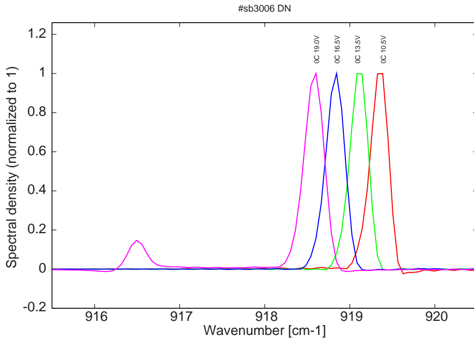
Figure 10: spectra at 0C for various LDD voltages (monomode up to 16.5V on LDD)
