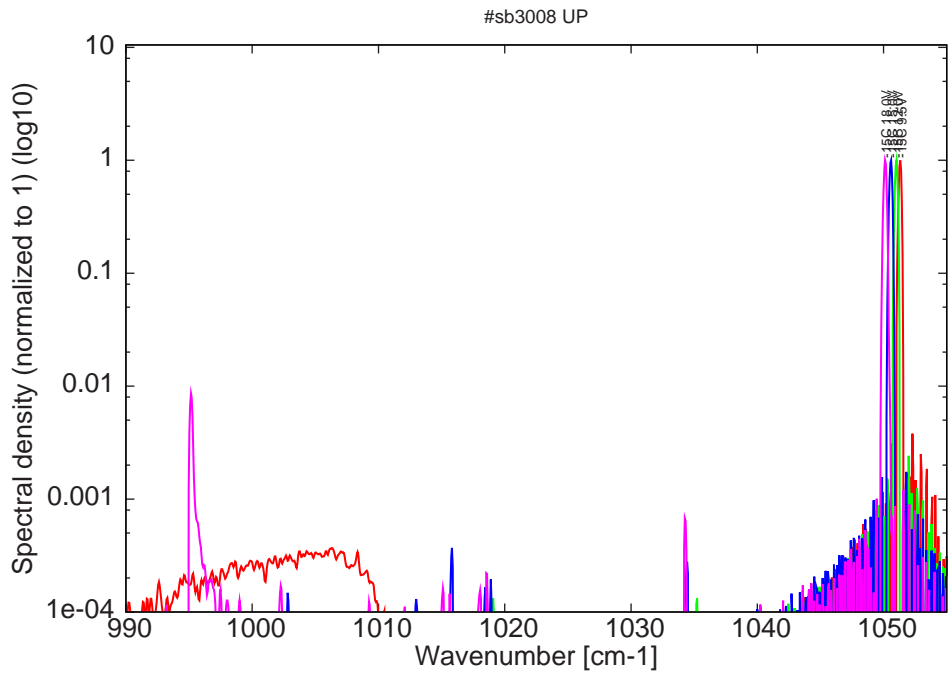
Figure 10: spectra at -15C for various LDD voltages (monomode up to 15V on LDD)
