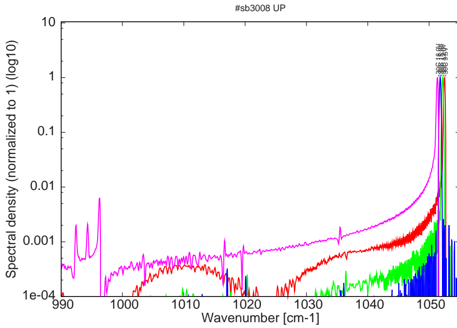
Figure 8: spectra at -30C for various LDD voltages (monomode up to 15V on LDD)
