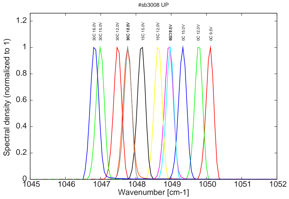
Figure 12: spectra at 0C, 15C and 30C for various LDD voltages (all monomode)
