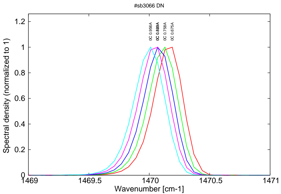
Figure 7: spectra at 0C at 2% duty-cycle, 20ns pulses on the laser (monomode range)
