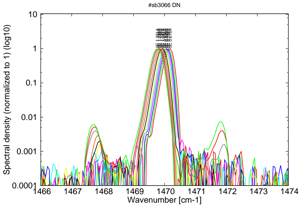
Figure 6: spectra at 0C at 2% duty-cycle, 20ns pulses on the laser (monomode up to 0.96A, then becomes multimode)
