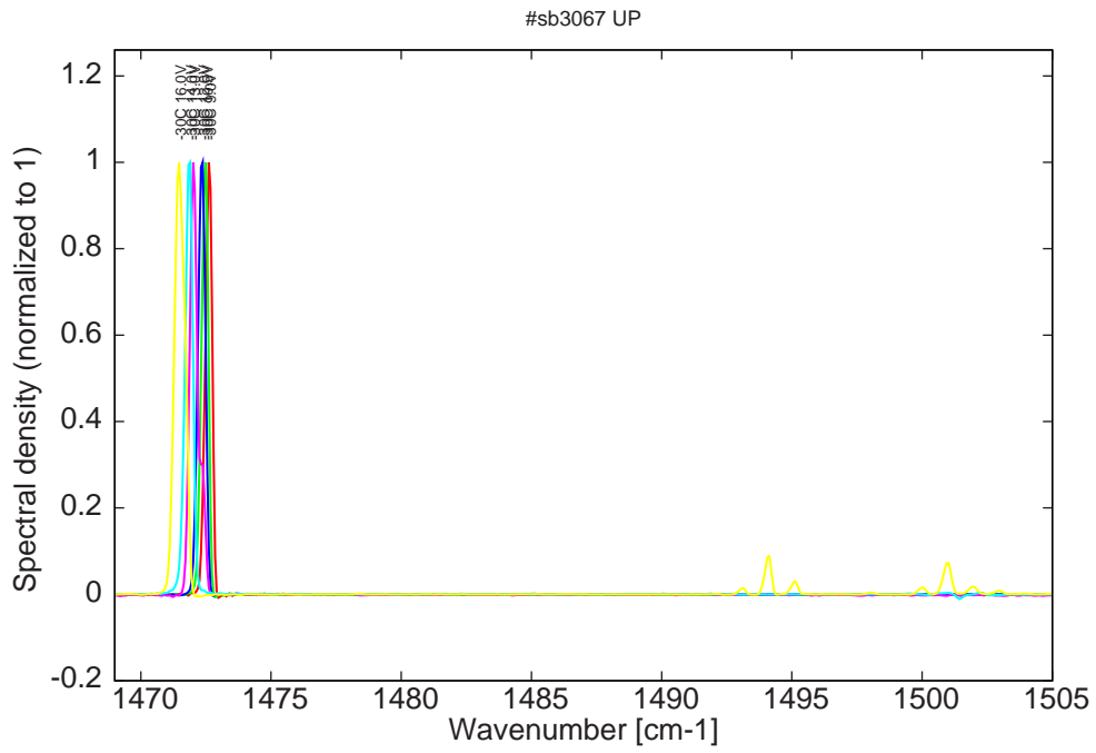
Figure 8: spectra at -30C for various LDD voltages (monomode up to 13V)
