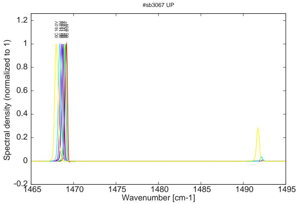
Figure 12: spectra at 0C for various LDD voltages (monomode up to 12V)
