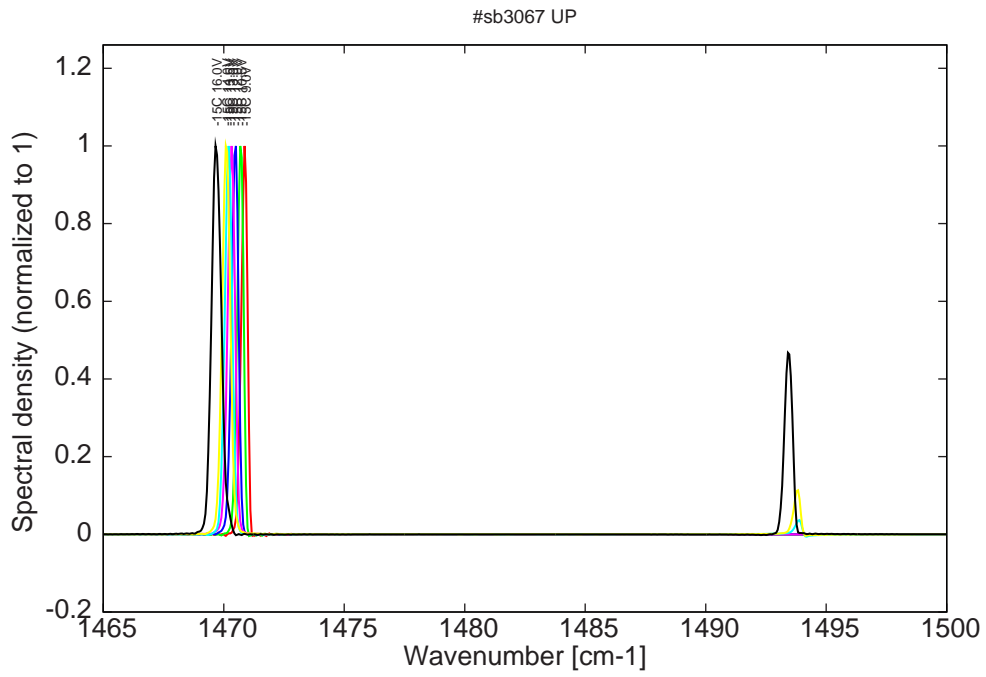
Figure 10: spectra at -15C for various LDD voltages (monomode up to 13V)
