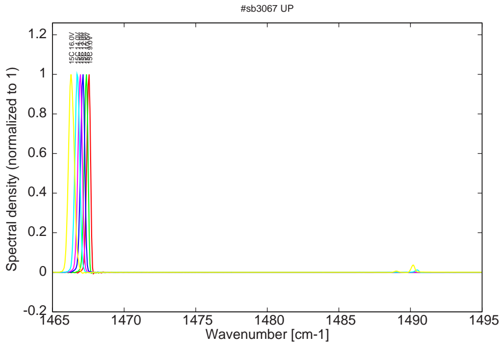
Figure 14: spectra at 15C for various LDD voltages (monomode up to 13V)
