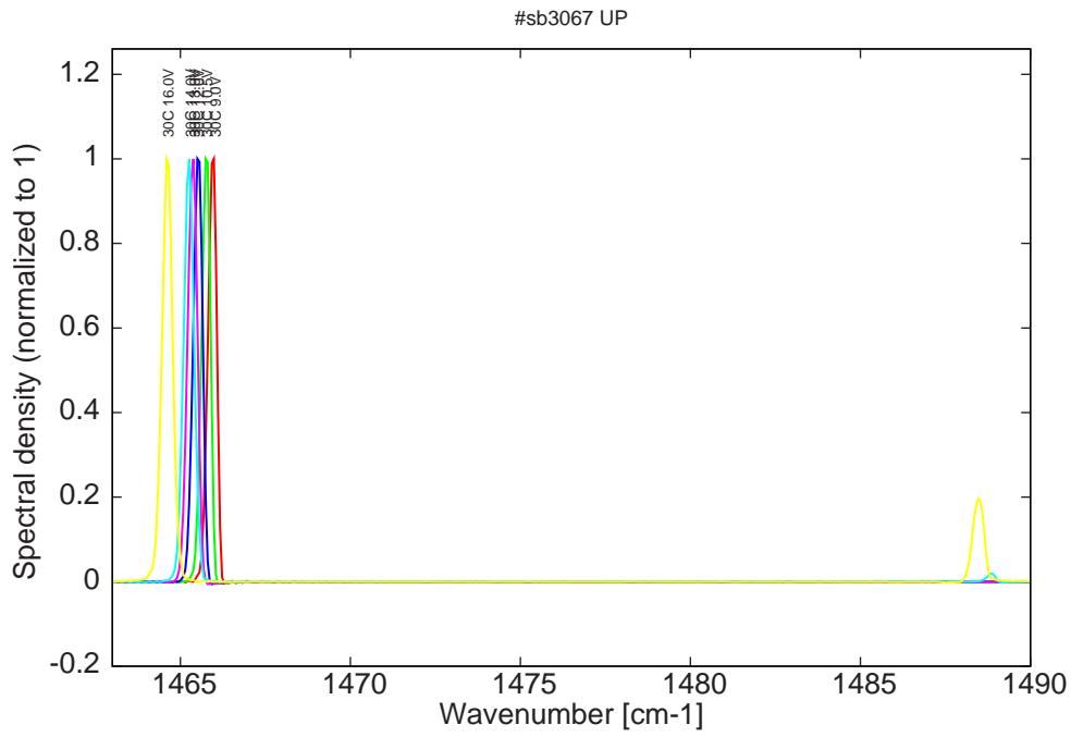
Figure 16: spectra at 30C for various LDD voltages (monomode up to 13V)
