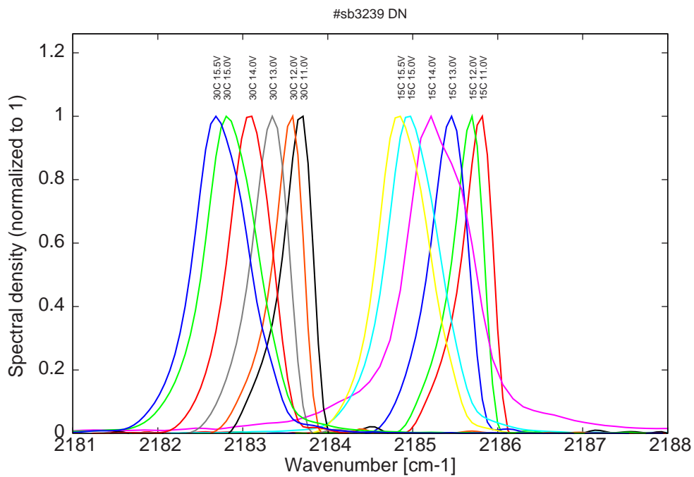
Figure 11: spectra between 15C and 30C for various LDD voltage (all monomode)
