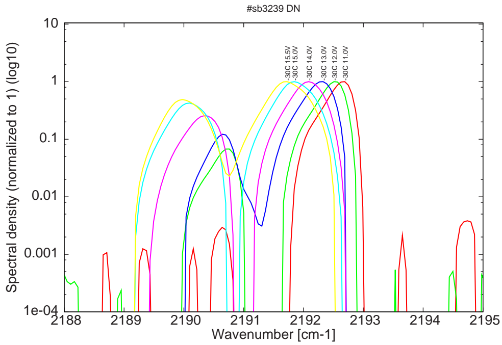
Figure 8: spectra at -30C for various LDD voltage (monomode only at threshold)
