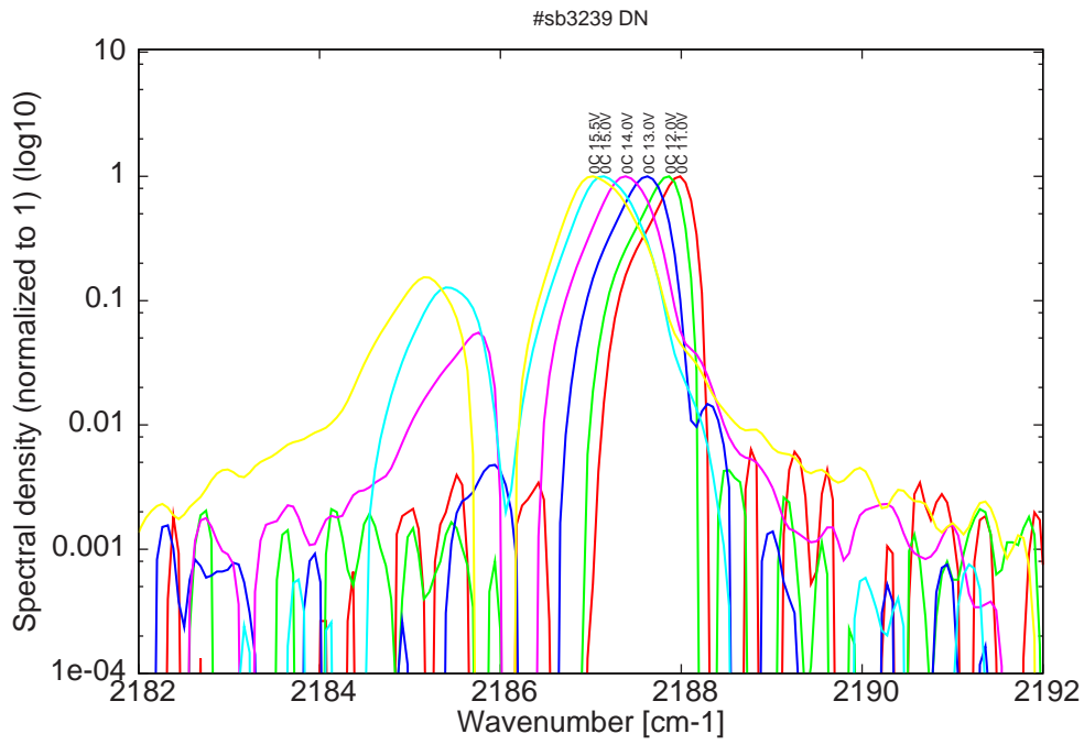
Figure 10: spectra at 0C for various LDD voltage (monomode up to 12.0V on LDD)
