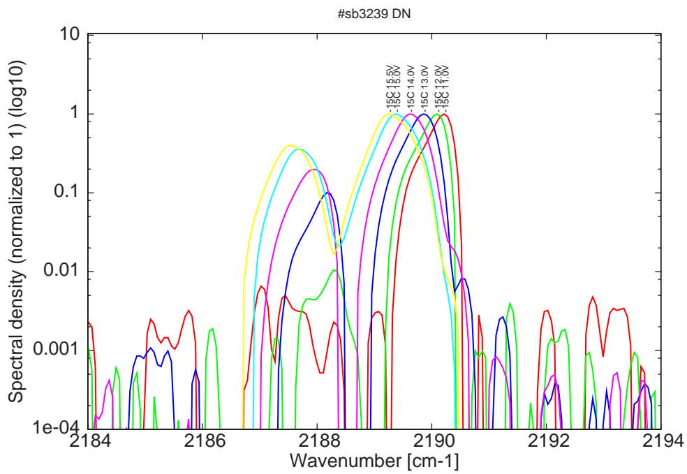
Figure 9: spectra at -15C for various LDD voltage (monomode only at threshold)
