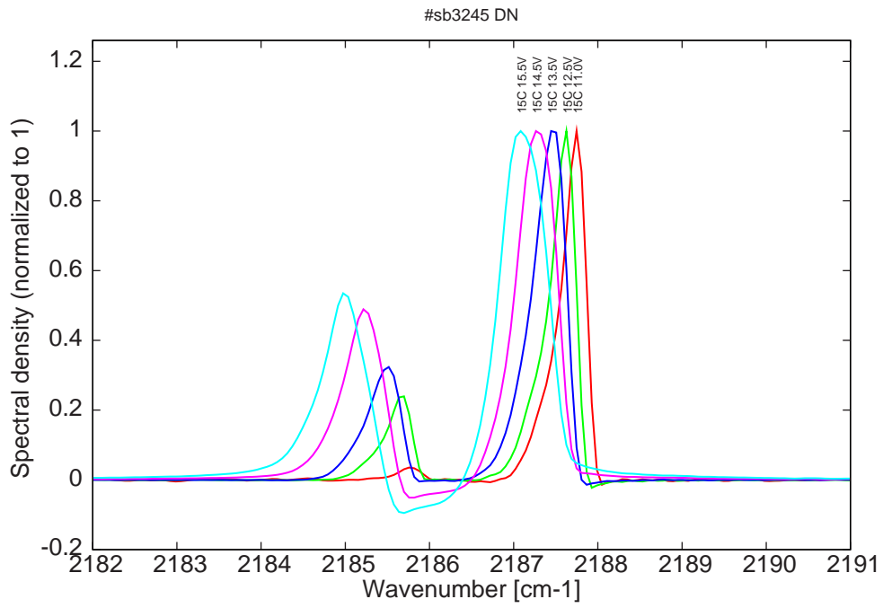
Figure 8: spectra at 15C for various LDD voltage (all bimode)
