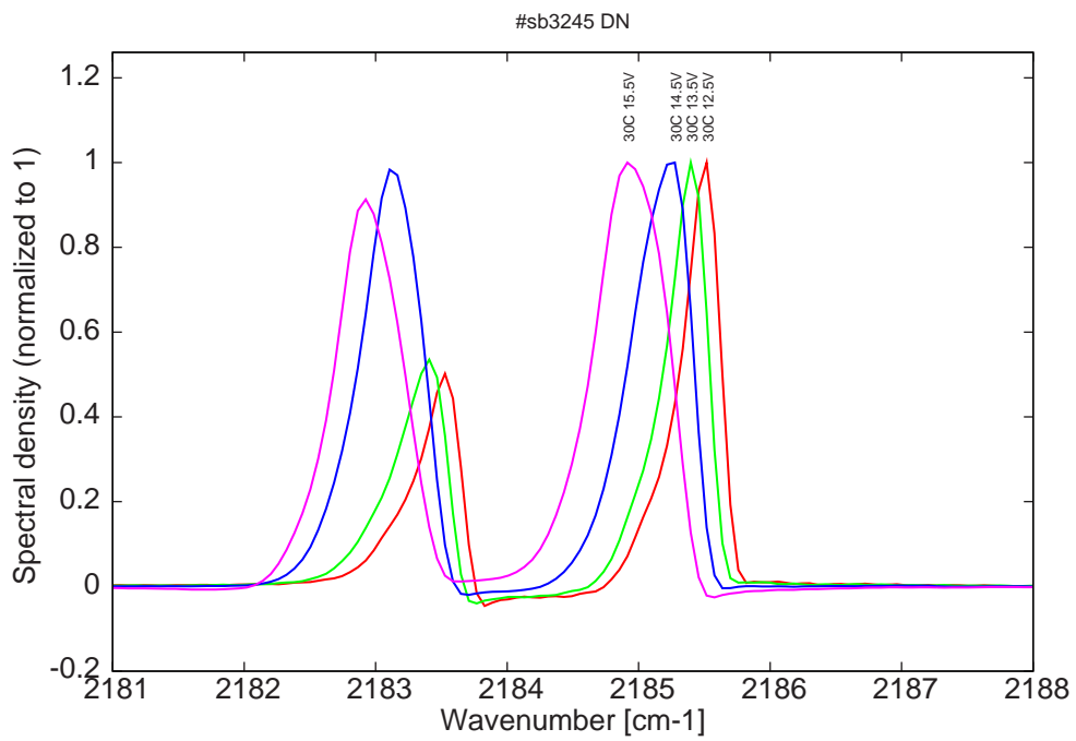
Figure 9: spectra at 30C for various LDD voltage (all bimode)
