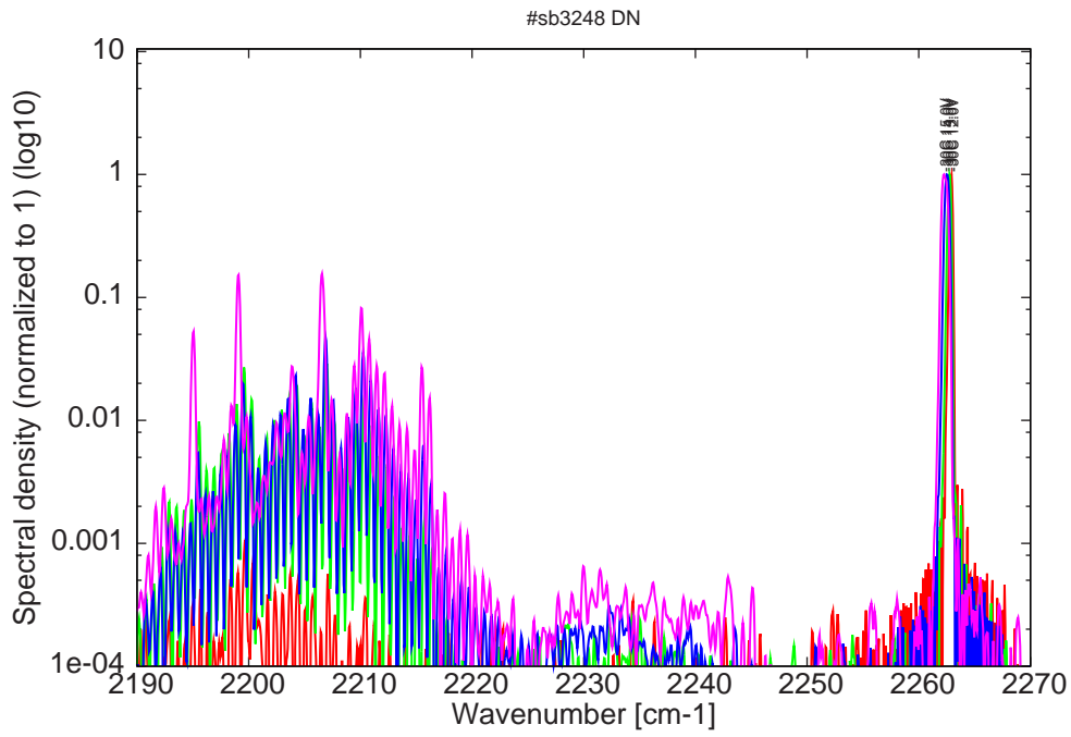
Figure 8: spectra at -30C for various LDD voltage (all multimode)
