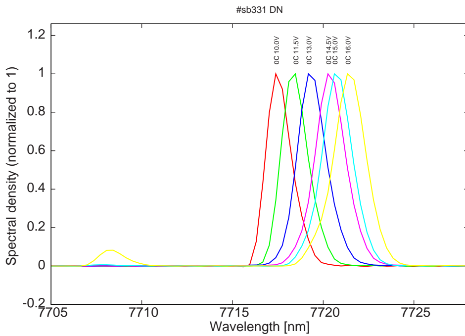
Figure 11: spectra at 0C for various LDD voltages (monomode - bimode)
