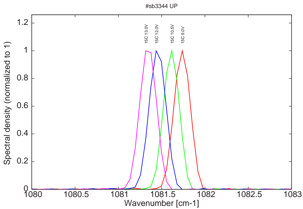
Figure 9: spectra at 15C for various LDD voltages (monomode range up to 13V on LDD, see Fig. 3)
