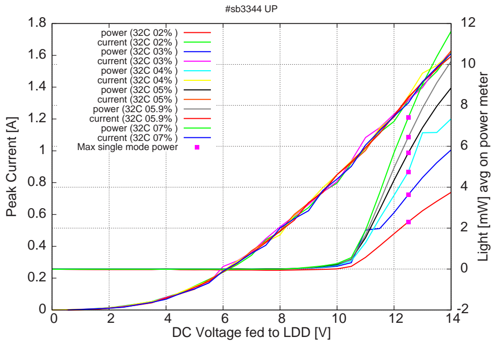
Figure 13: peak current and average power vs LDD voltage at 32C for various duty-cycles (100ns pulses on the laser)
