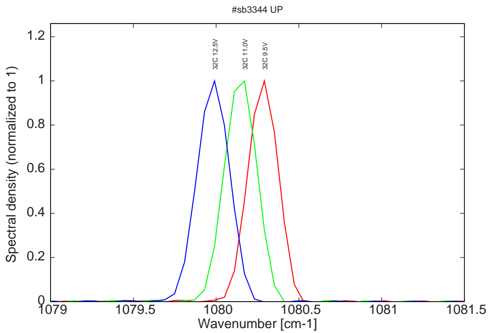
Figure 11: spectra at 32C for various LDD voltages (monomode range up to 12.5V on LDD, see Fig. 3)
