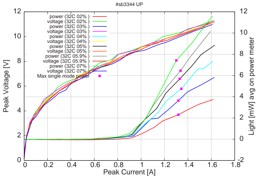
Figure 12: peak voltage and average power vs peak current at 32C for various duty-cycles (100ns pulses on the laser)
