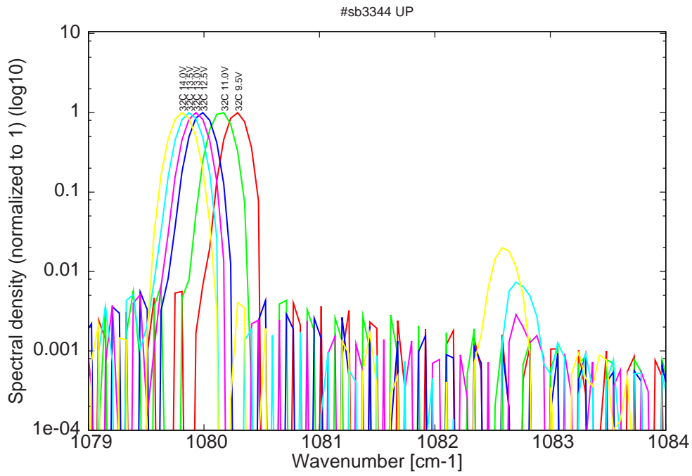
Figure 10: spectra at 32C for various LDD voltages (22ns pulses, 1.1us period)
