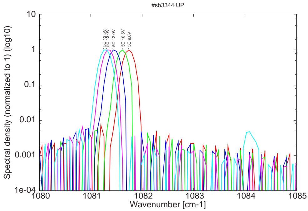
Figure 8: spectra at 15C for various LDD voltages (22ns pulses, 1.1us period)
