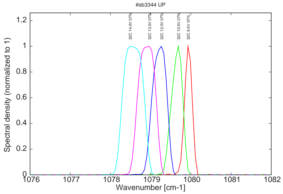
Figure 14: spectra at 32C at 7% duty-cycle for various LDD voltages (all monomode)
