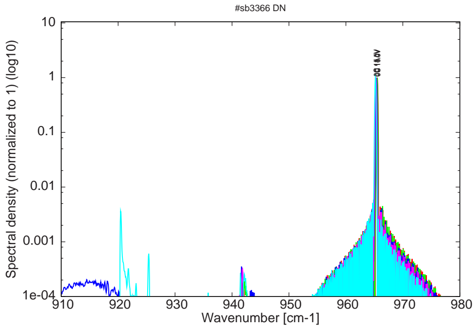
Figure 12: spectra at 0C for various LDD voltages (monomode up to 14V on LDD)
