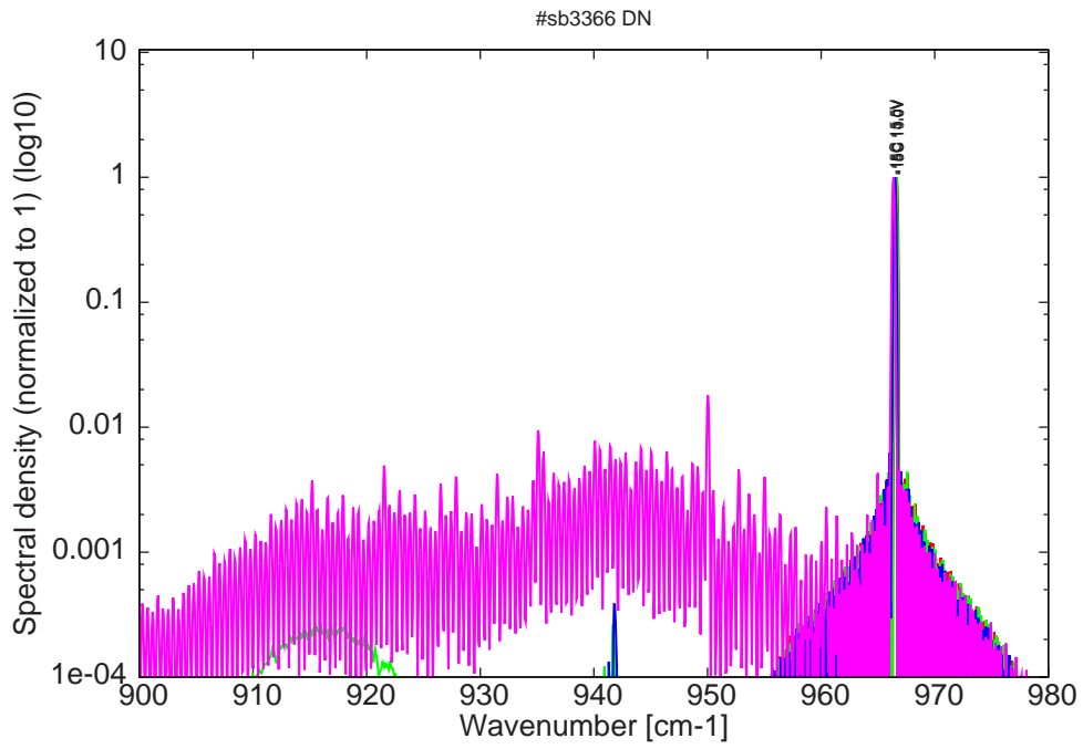
Figure 10: spectra at -15C for various LDD voltages (monomode up to 13V on LDD)
