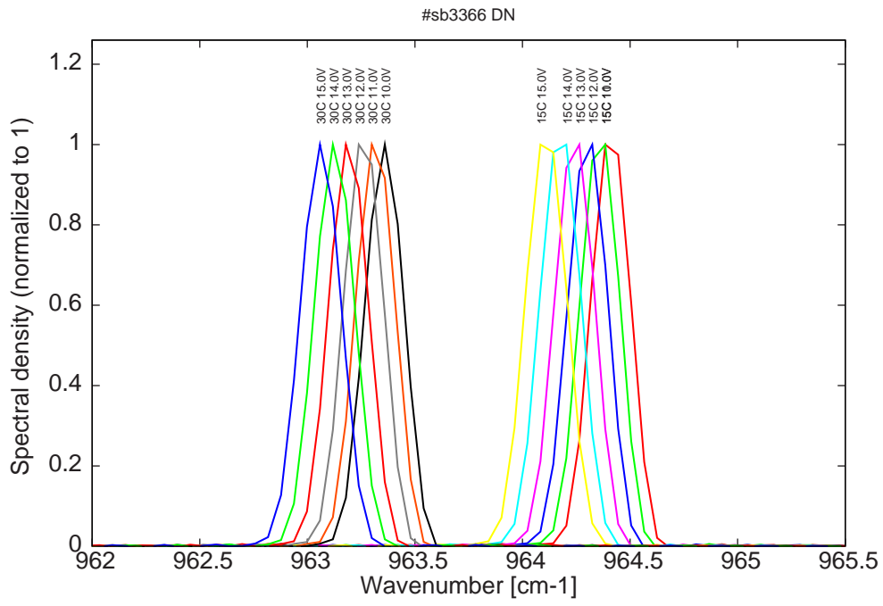
Figure 14: spectra at 15C and 30C for various LDD voltages (all monomode)
