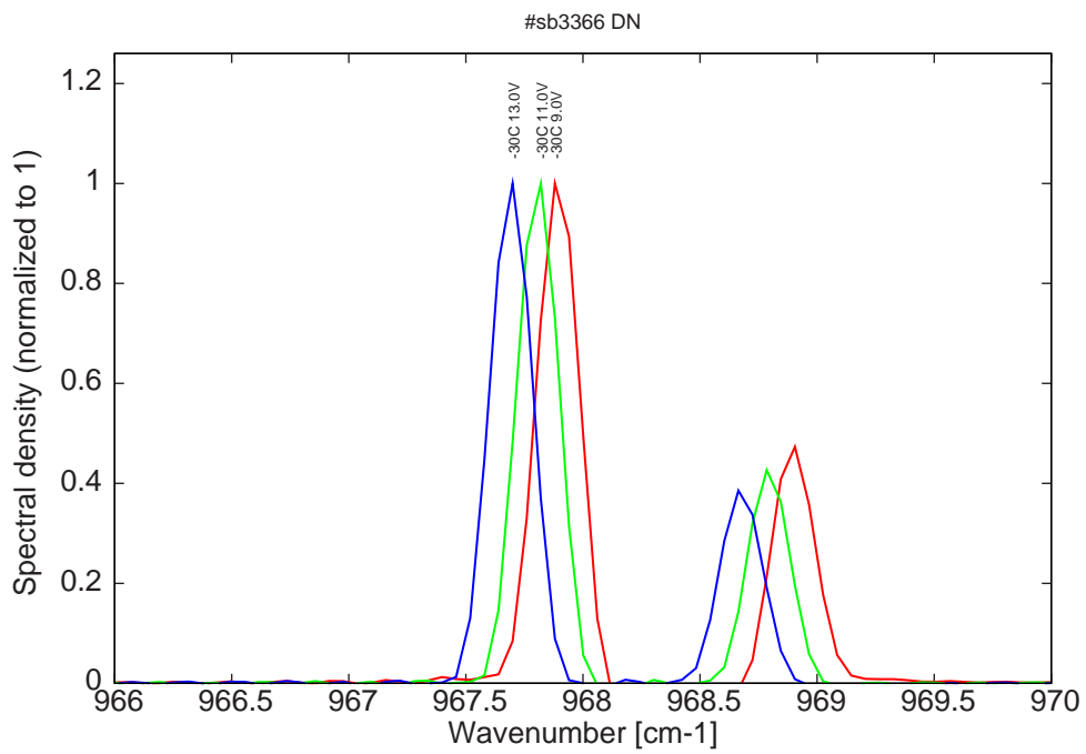
Figure 9: spectra at -30C for various LDD voltages (all bimode)
