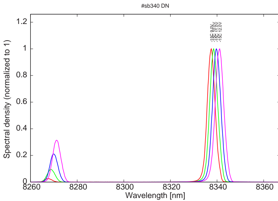
Figure 10: spectra at -15C for various LDD voltages (all bimode)
