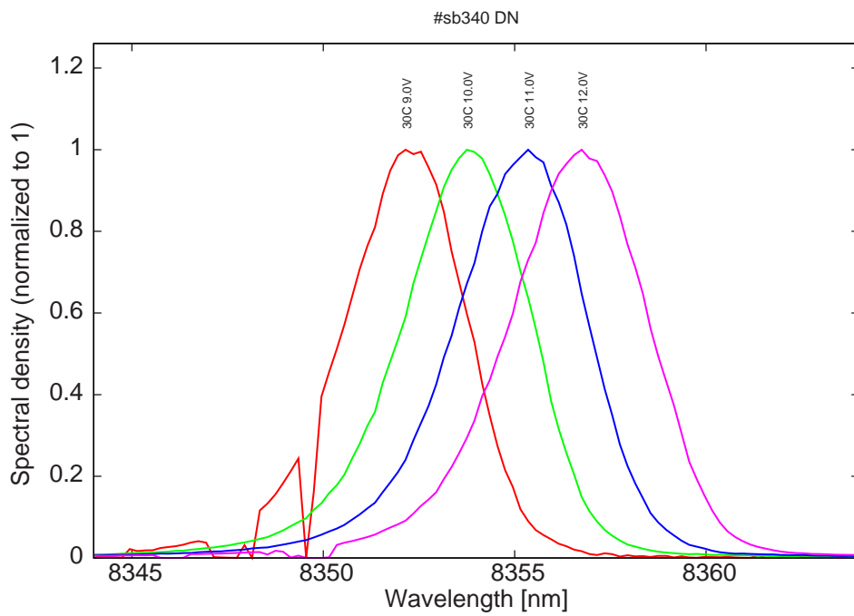
Figure 14: spectra at 30C for various LDD voltages (all monomode)
