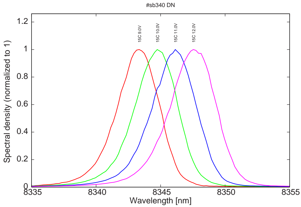
Figure 13: spectra at 15C for various LDD voltages (all monomode)
