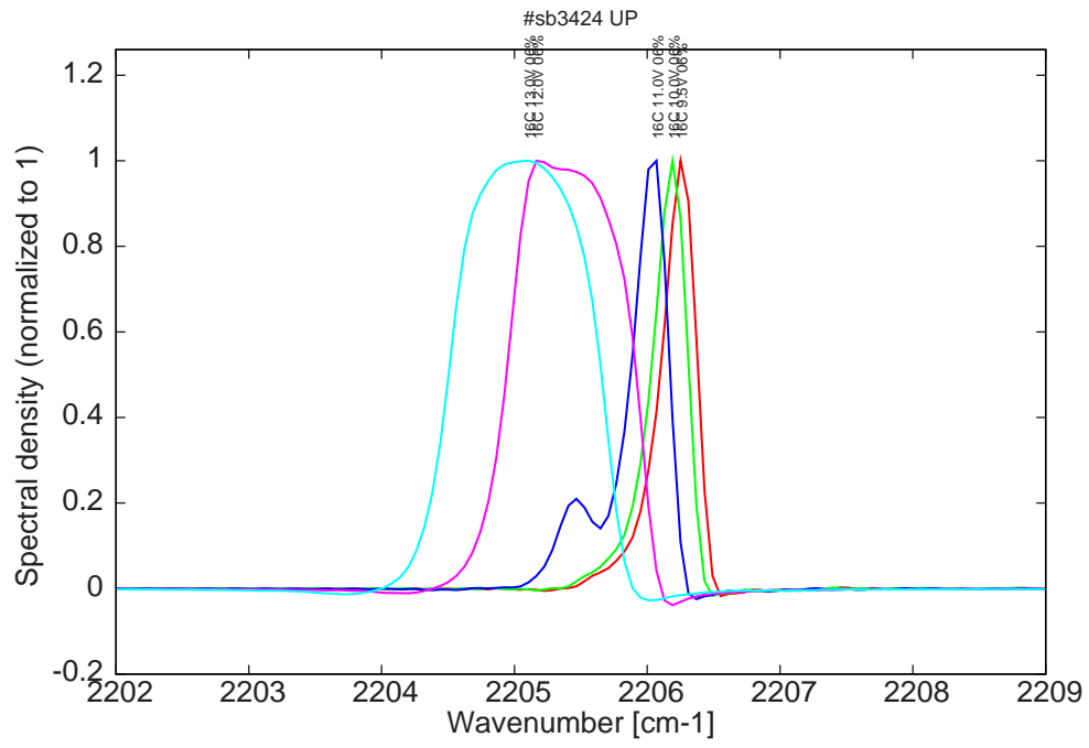
Figure 8: spectra at 16C at 6% duty-cycle for various LDD voltages
