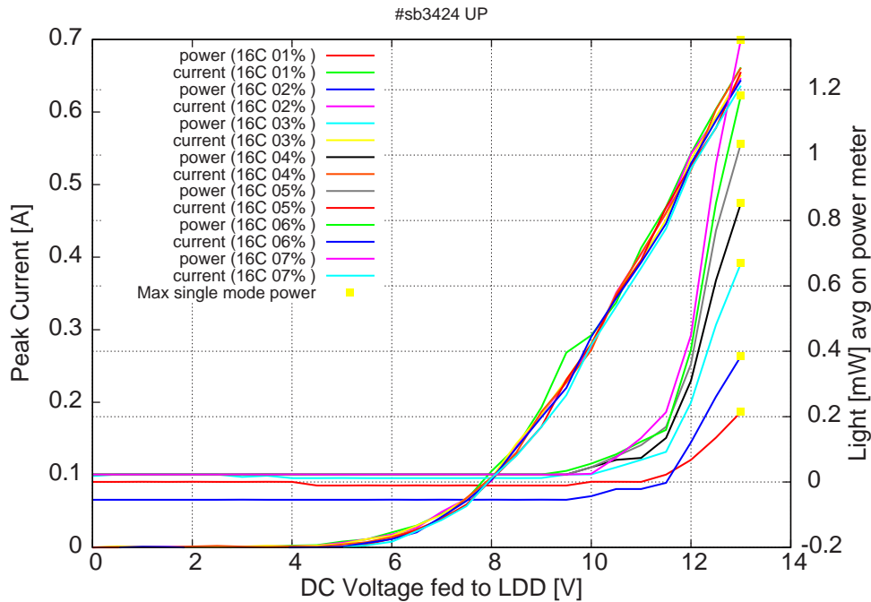
Figure 7: peak current and average power vs LDD voltage at 16C for various duty-cycles (100ns pulses on the laser) (the solid squares indicate the maximum singlemode emitted power)
