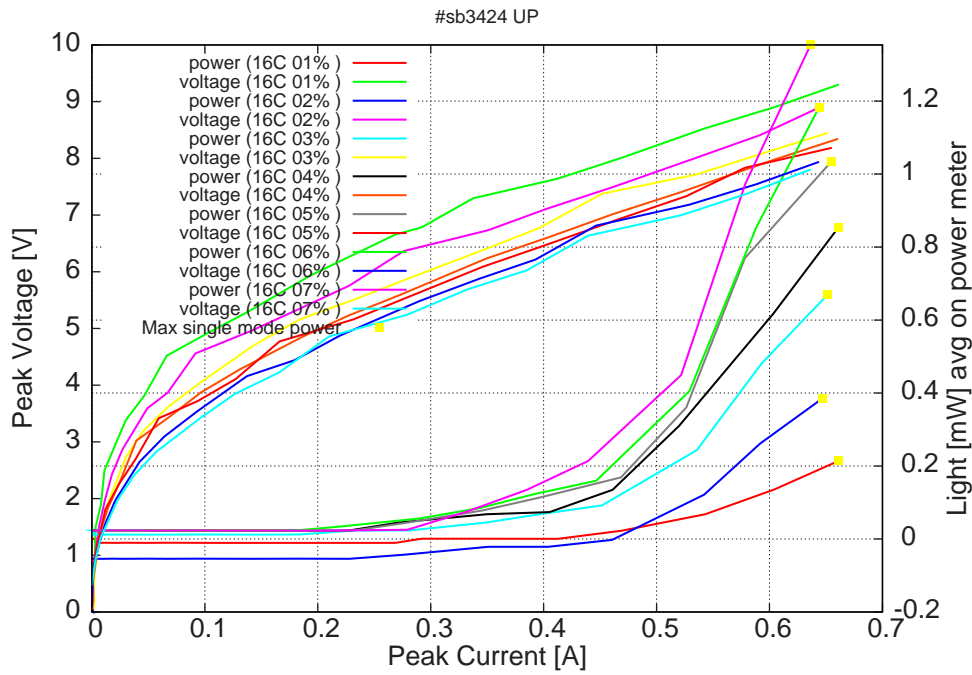
Figure 6: peak voltage and average power vs peak current at 16C for various duty-cycles (100ns pulses on the laser) (the solid squares indicate the maximum singlemode emitted power)
