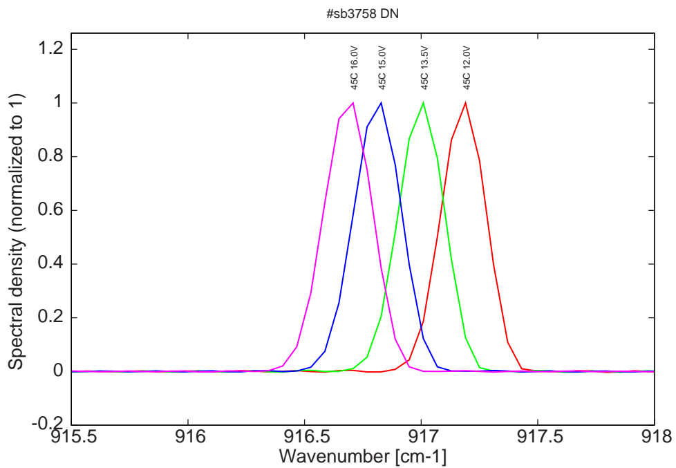
Figure 9: spectra at 45C for various LDD voltages (all monomode)
