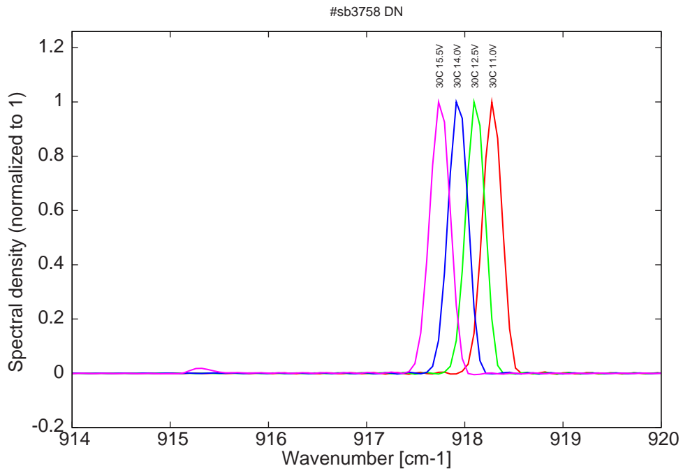
Figure 8: spectra at 30C for various LDD voltages (monomode up to 14.0V on LDD)
