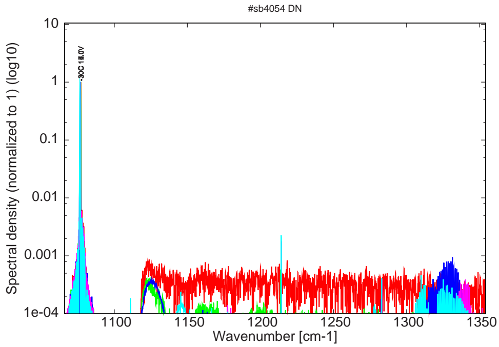
Figure 8: spectra at -30C for various LDD voltages (monomode, then becomes multimode for LDD voltage > 12V)
