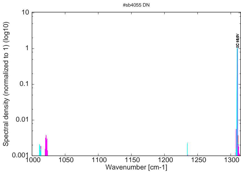
Figure 11: spectra at 0C for various LDD voltages (monomode on mode 2, then becomes multimode for LDD voltage >13V)
