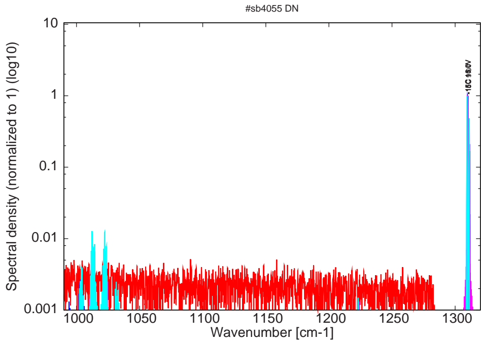
Figure 10: spectra at -15C for various LDD voltages (all multimode)
