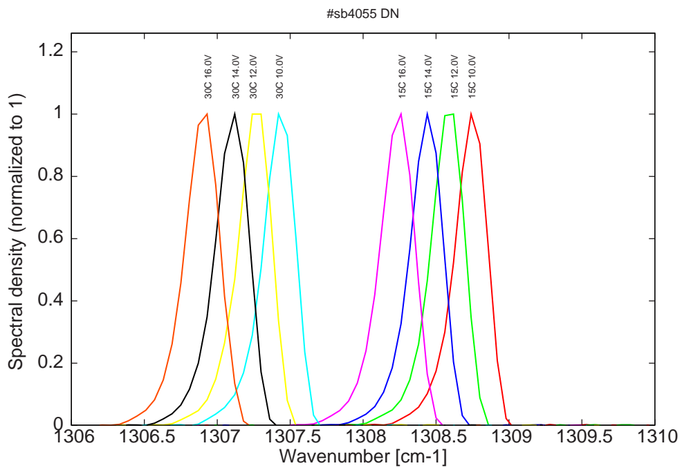
Figure 13: spectra at 15C and 30C for various LDD voltages (monomode on mode 2)
