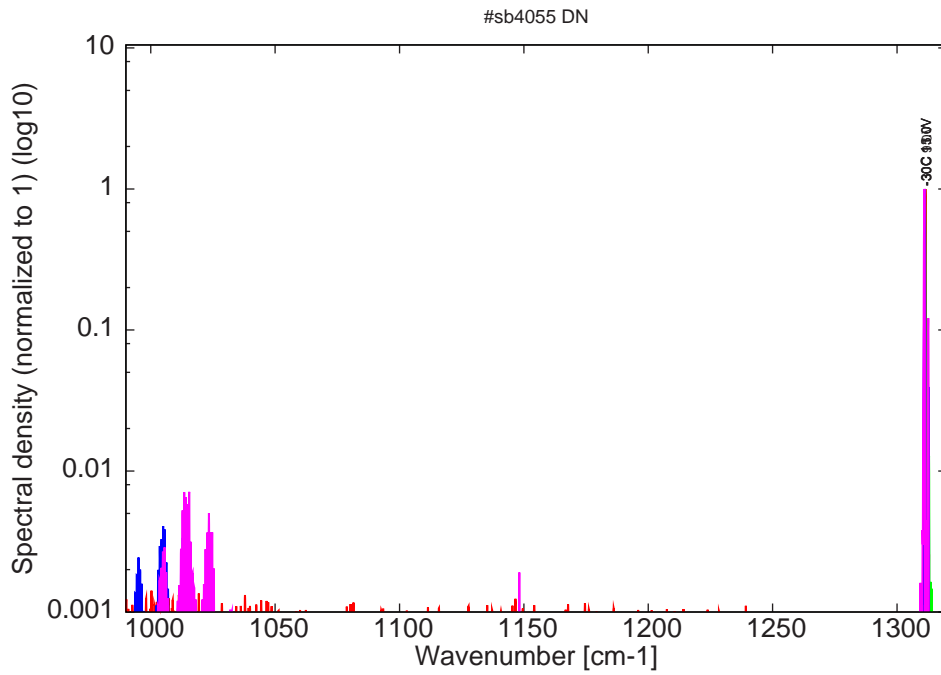
Figure 8: spectra at -30C for various LDD voltages (monomode on mode 1, then becomes multimode for LDD voltage > 11V)
