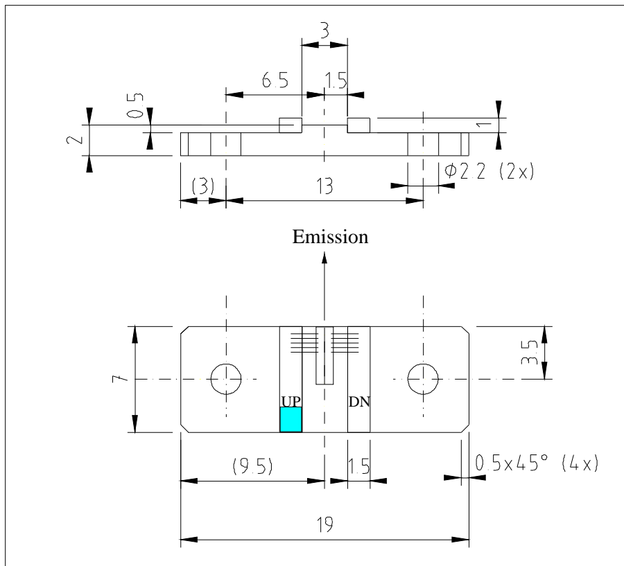
Figure 1: Mechanical and electrical interface for #sb468 UP (please note that the laser is connected to the UP pad drawn in blue)
