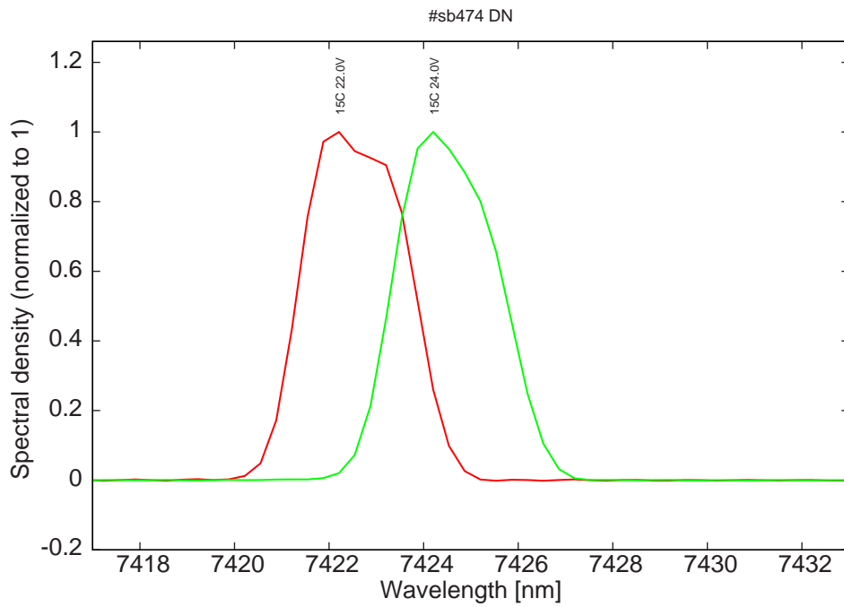
Figure 16: spectra at 15C for various LDD voltages (monomode range, but with mode jumping compared to spectra at 0C)
