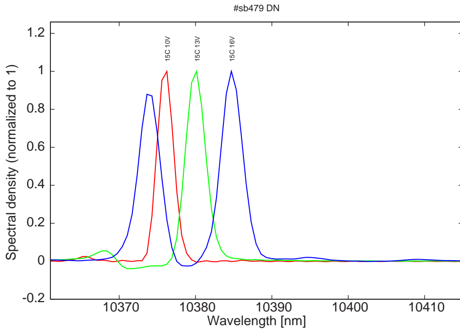
Figure 15: spectra at 15C for various LDD voltages (all multimode)
