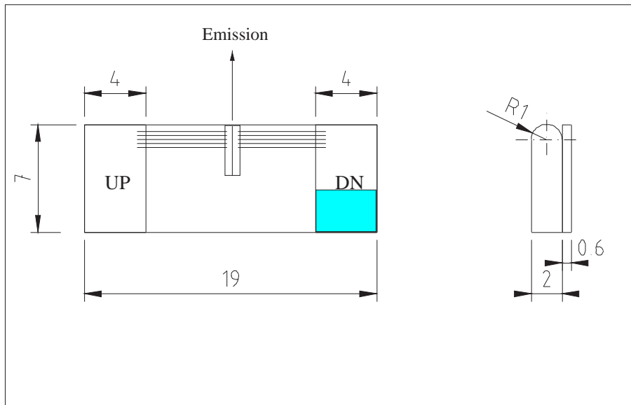
Figure 1: Support mounting for #sb479 DN (please note that the laser is connected to the DN pad drawn in blue)
