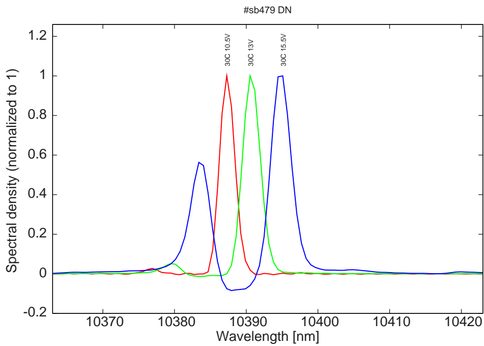
Figure 16: spectra at 30C for various LDD voltages (all multimode)
