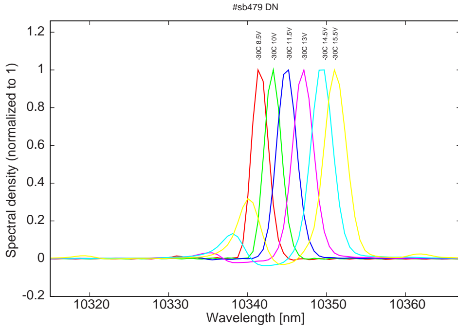
Figure 9: spectra at -30C for various LDD voltages (small mode around 10318 nm)
