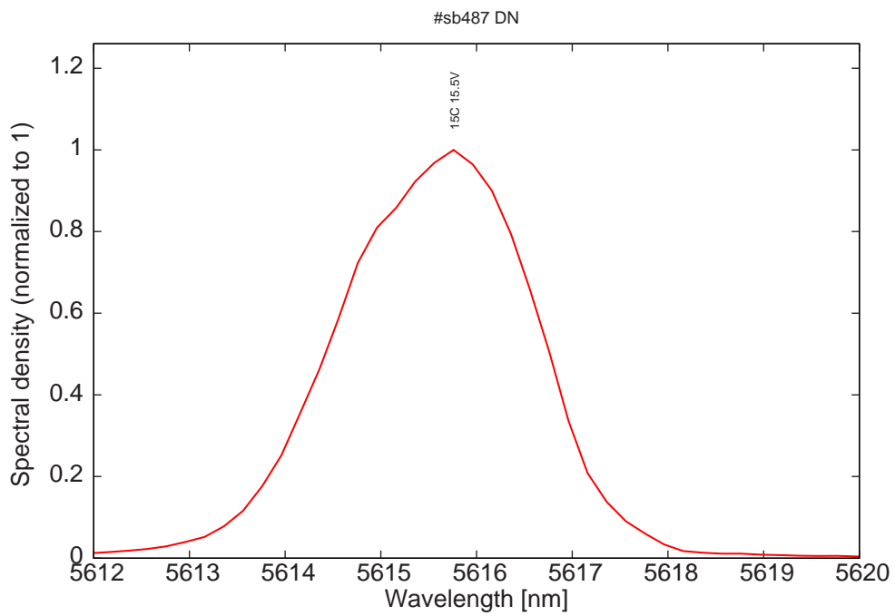
Figure 16: monomode spectrum at 15C at 15.5V on LDD
