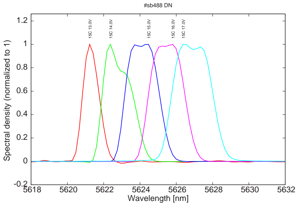
Figure 10: spectra at 15C at 2% dc (50ns pulses, 2.5 \mu s period) for various LDD voltages (spectra shape due to pulses length)
