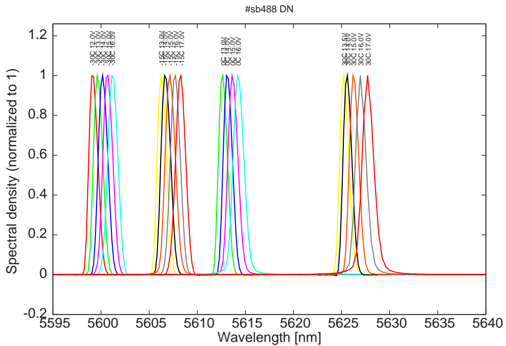
Figure 6: spectra at -30C, -15C, 0C and 30C at 2% dc (22ns pulses, 1.1 \mu s period) for various LDD voltages
